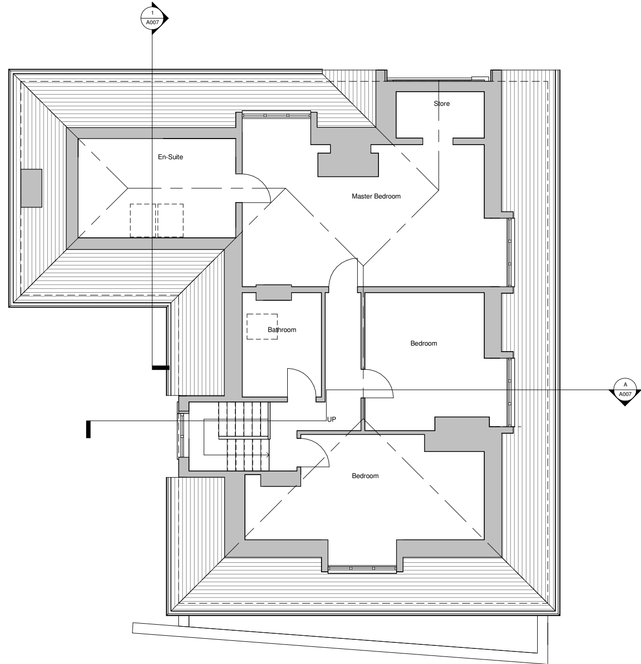
Second Floor 1 : 50
