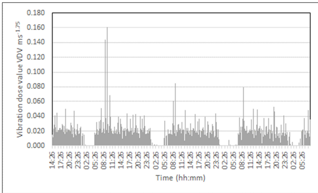
Figure 9: Measured z-axis vibration dose values (VDV \text{ms}^{-1.75} )
