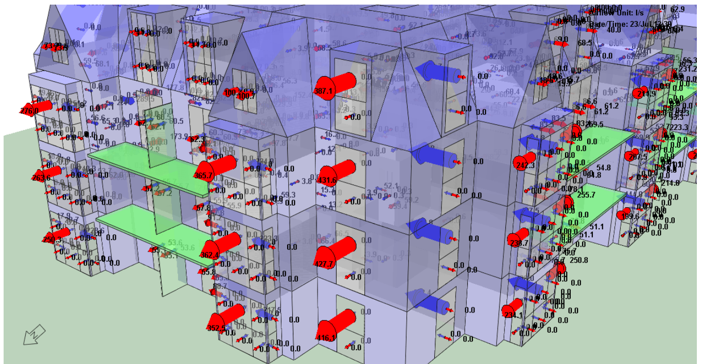
Figure 8. IES-VE Thermal Model - MacroFlo Natural Ventilation
