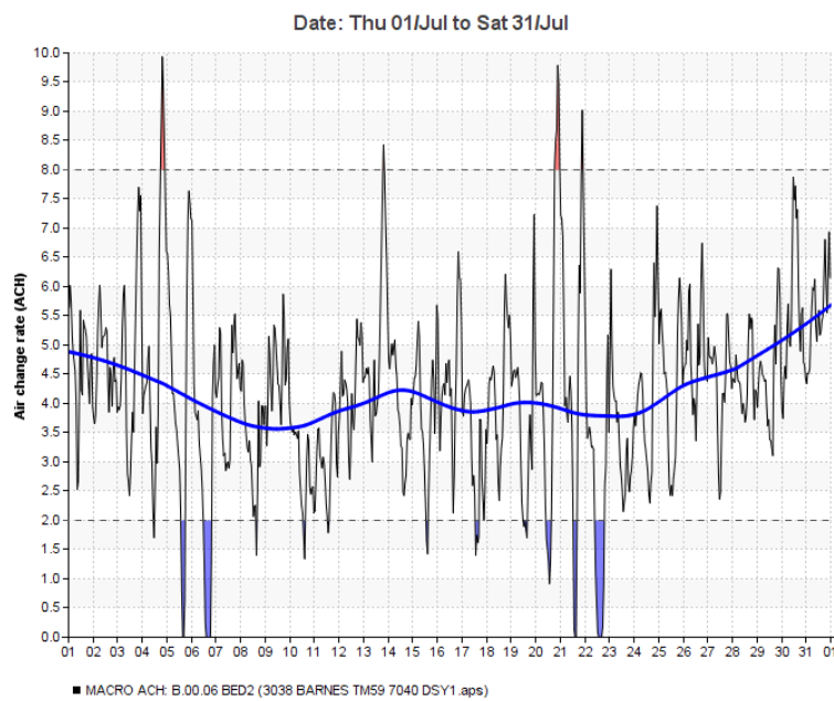
Figure 10. Natural Ventilation Bulk Air Movement, Typical Bedroom
