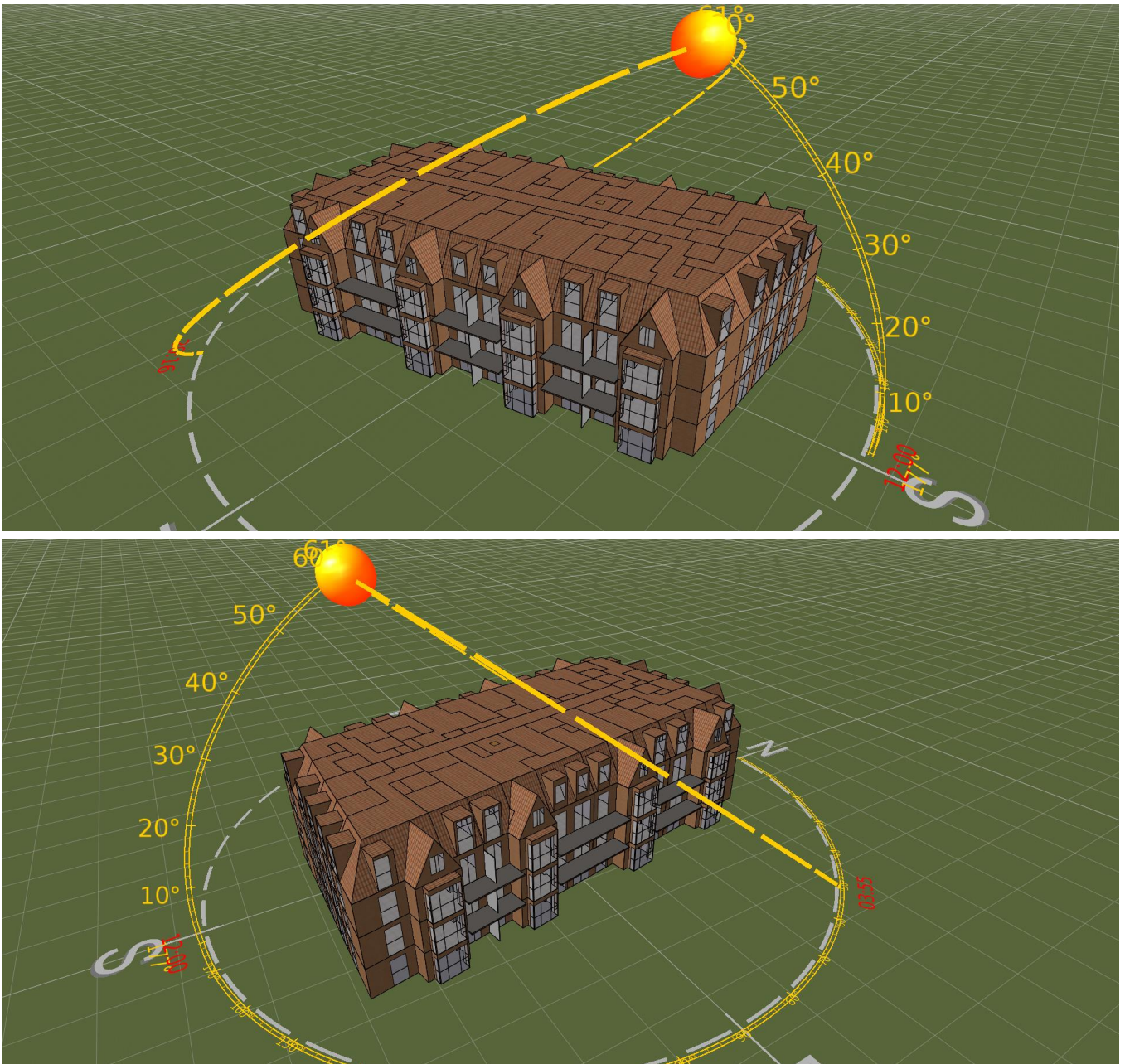
Figure 7. IES-VE Thermal Model Image
