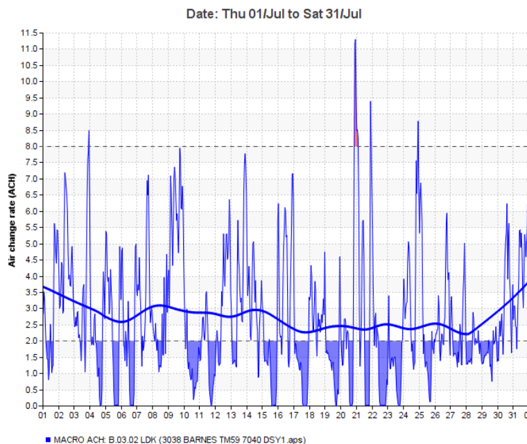
Figure 11. Natural Ventilation Bulk Air Movement, Typical LDK
