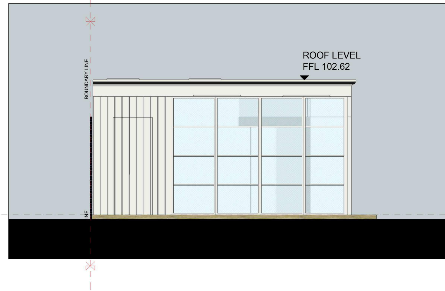
FRONT ELEVATION
