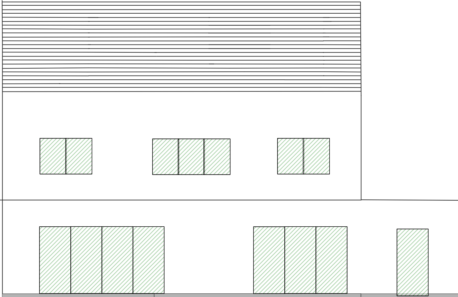
Proposed REAR VIEW 1:50
