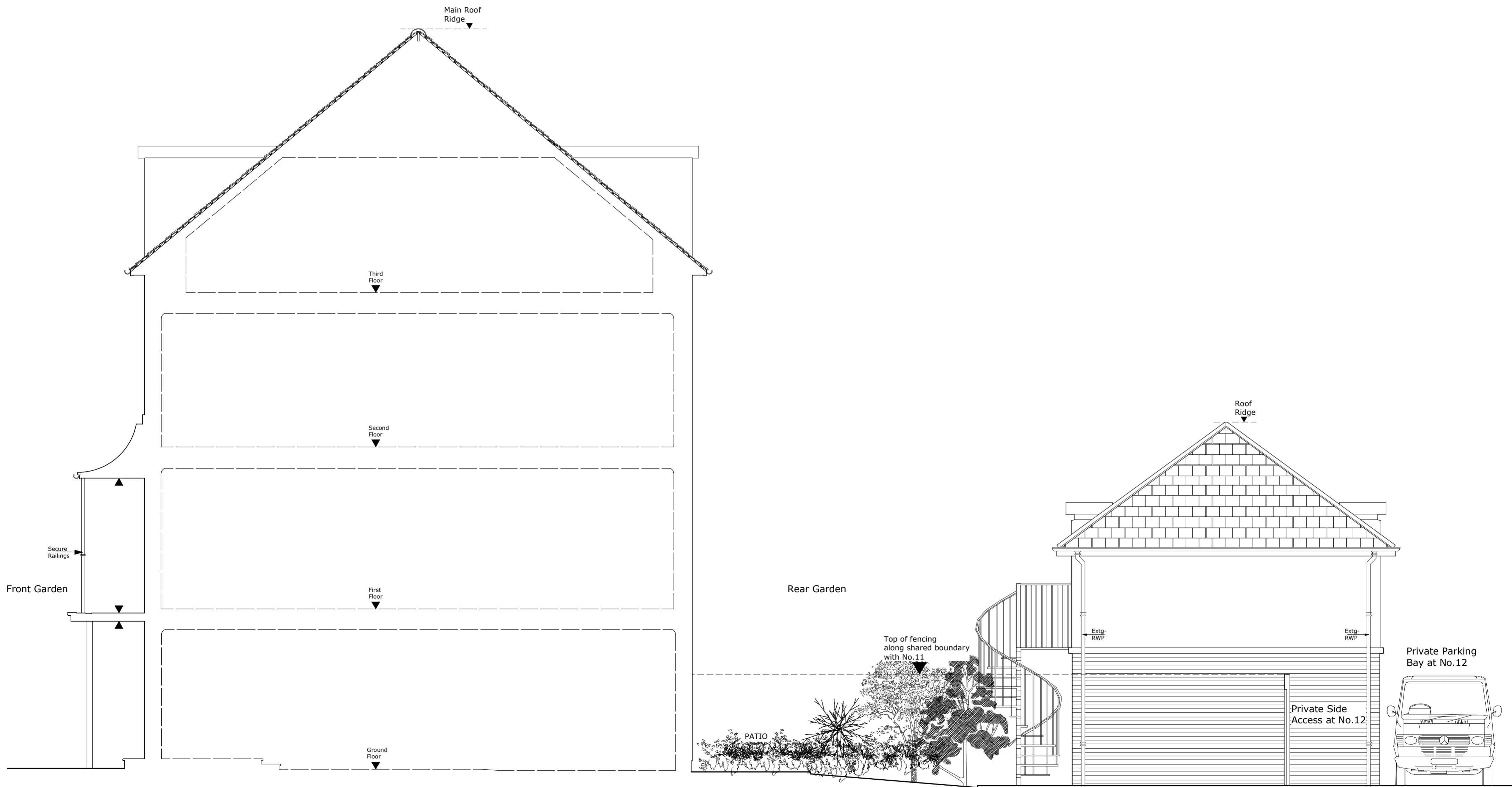
c Side Elevation/Section 14 Existing Layout
