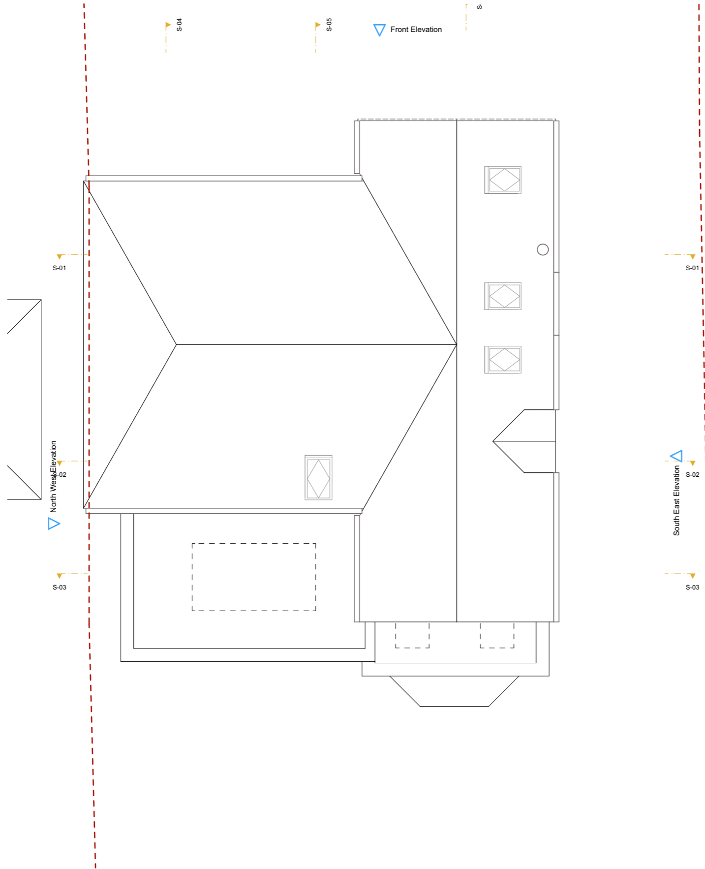
Roof Plan 1:100
