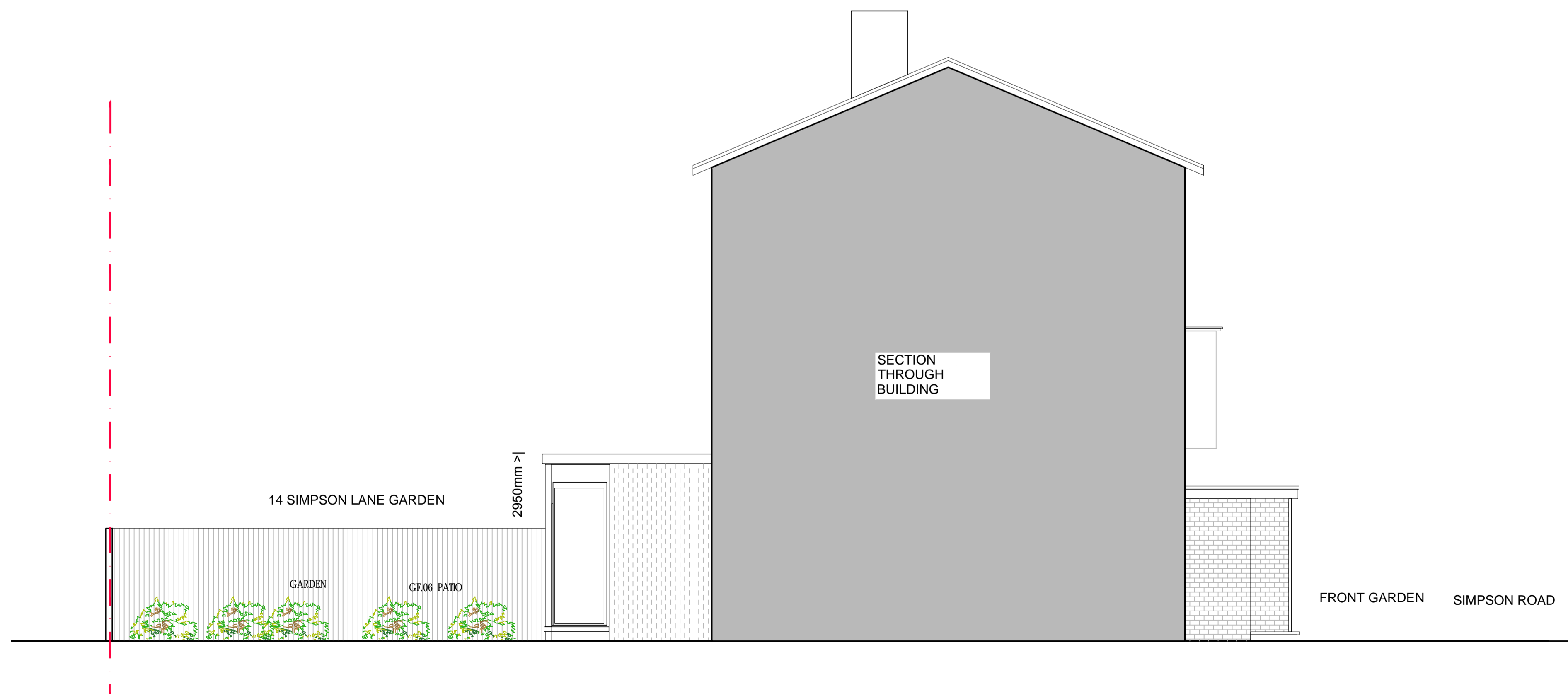
2 Proposed Flank (East) Elevation
