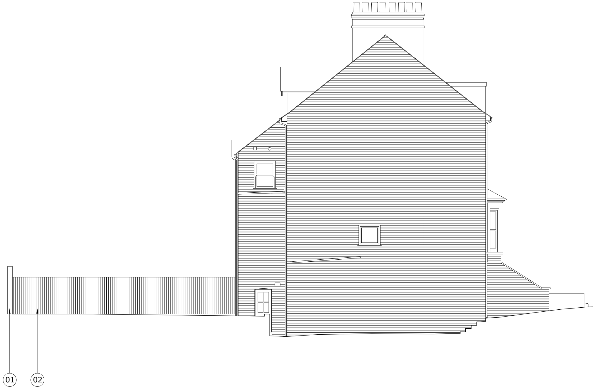
01 Existing_Side Elevation 01 301 Scale 1:100@A3
