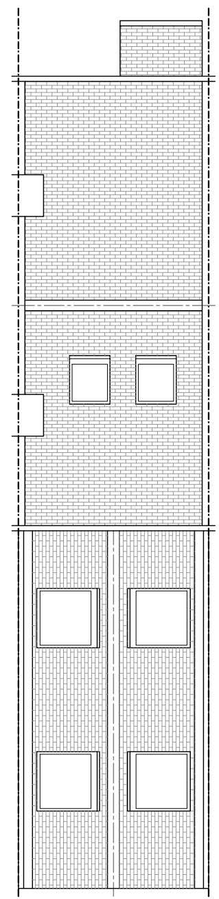
Proposed Roof Plan Scale 1/100@A3
