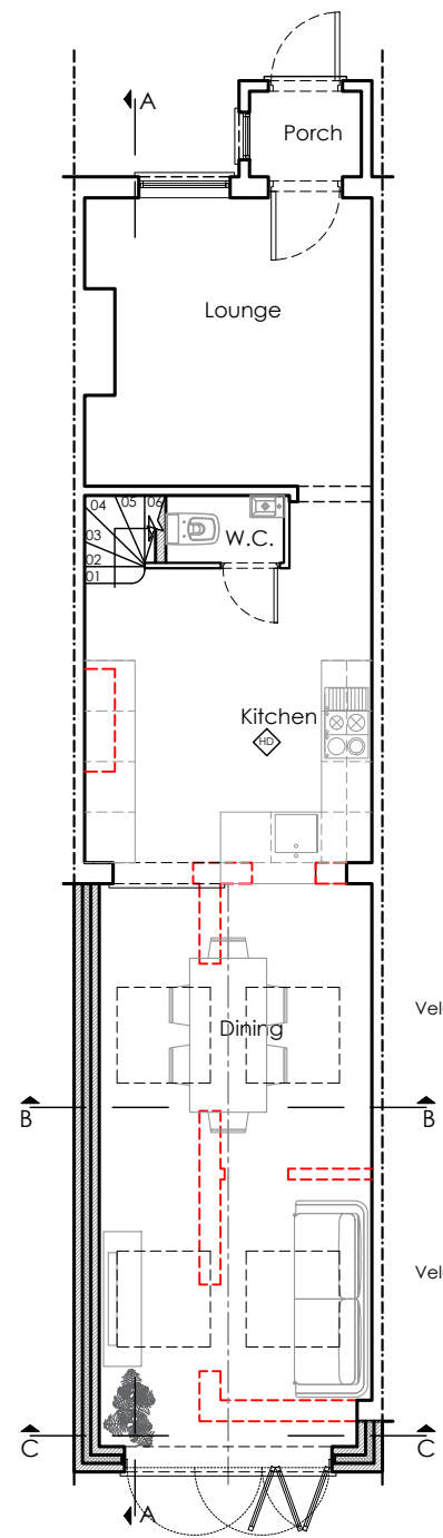
Proposed Ground Floor Plan Scale 1/100@A3
