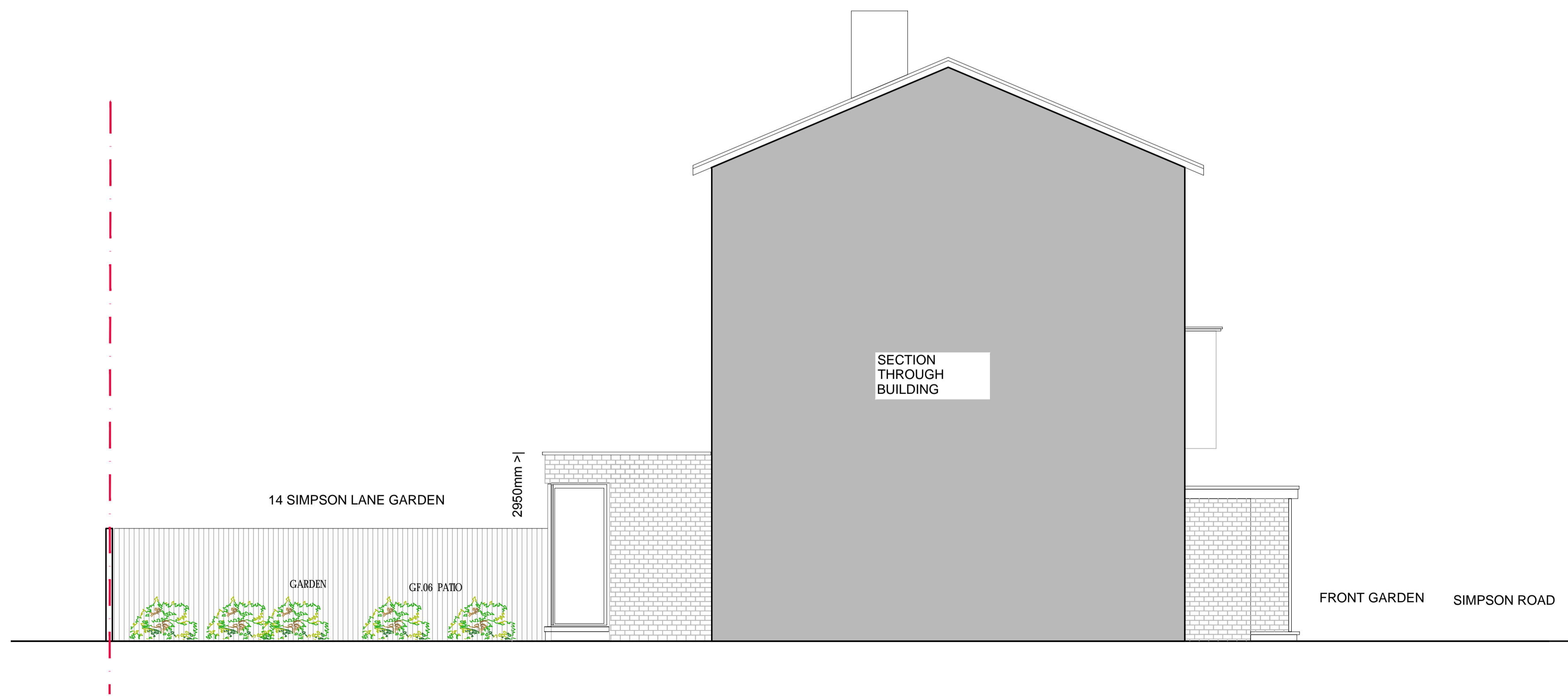
2 Proposed Flank (East) Elevation Scale: 1:100 @ A3
