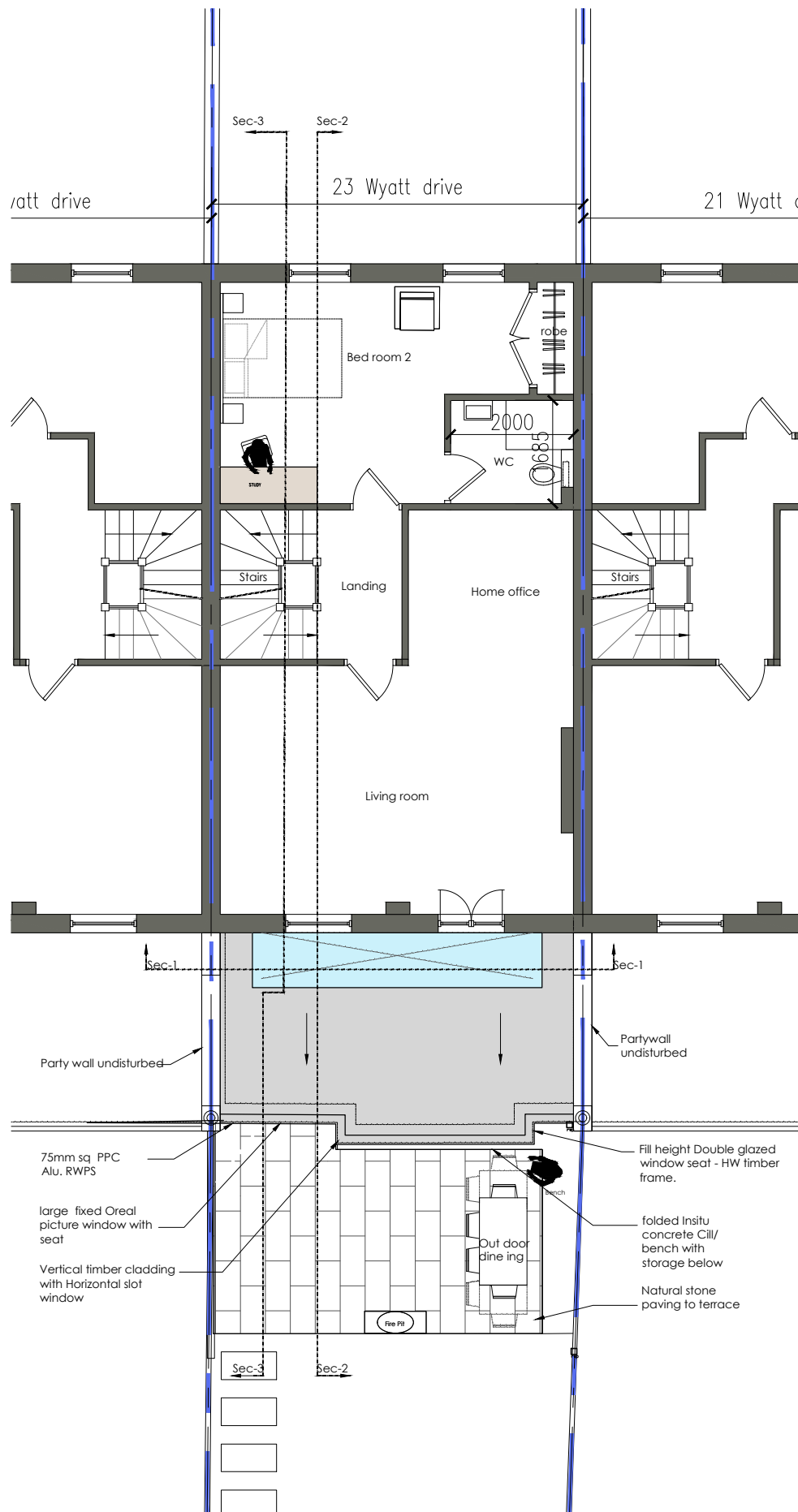
1st floor plan SCALE - 1:100 Proposed
