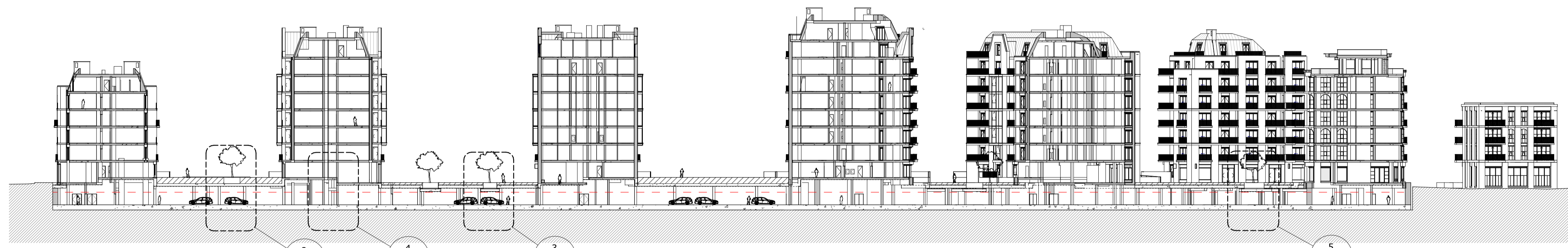
1 Basement Section_Phase 01_002 1 : 500
