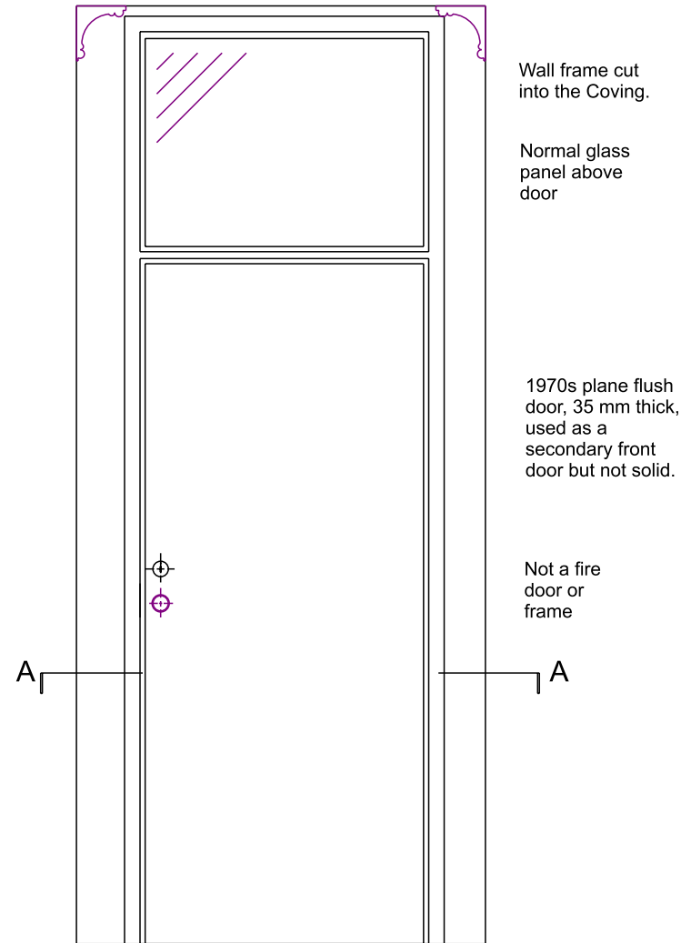
Landing Side of Elevation
