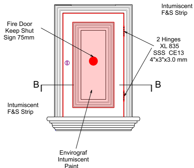
Door "E" Corridor Elevation
