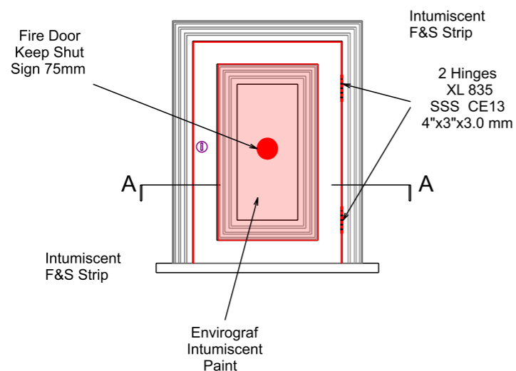
Door "B" Corridor Elevation
