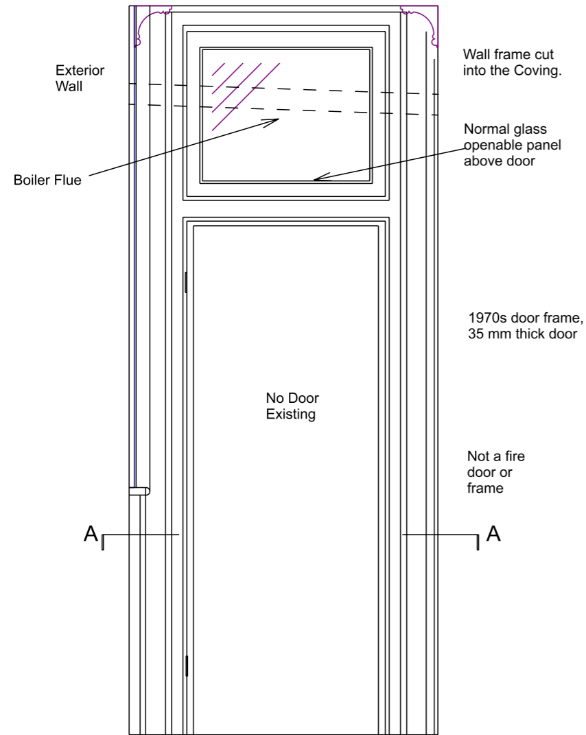
F005 Side of Elevation
