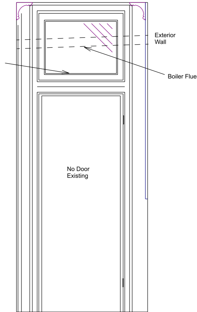
F008 Side of Elevation
