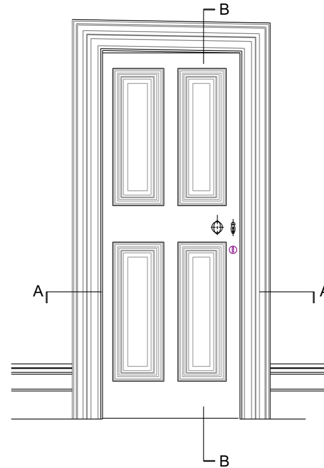
Corridor Side Elevation
