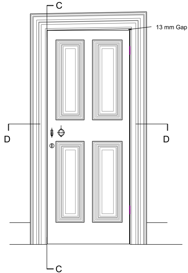
Room Side Elevation
