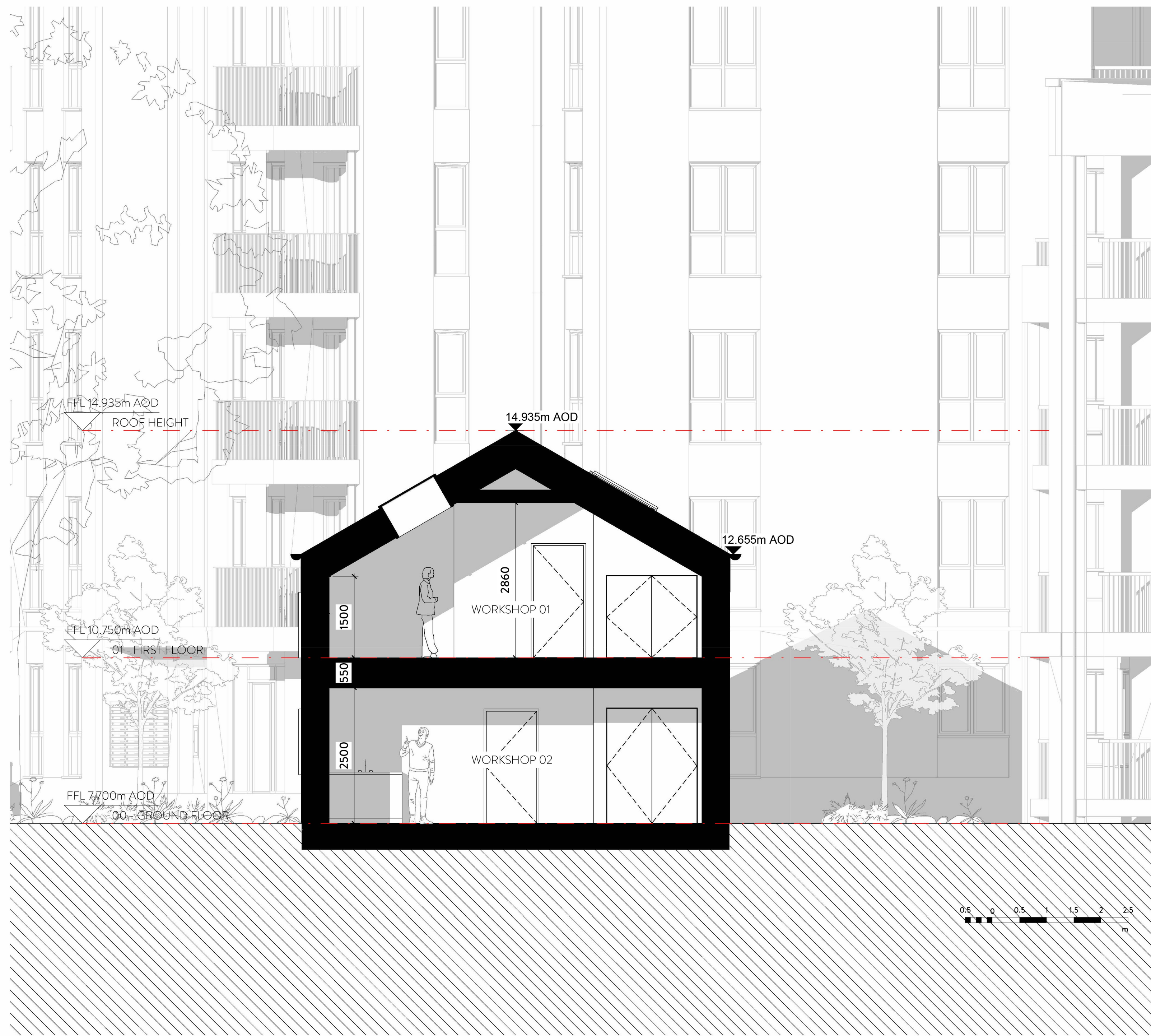
1 PROPOSED SECTION A-A - 1:50 @ A1
