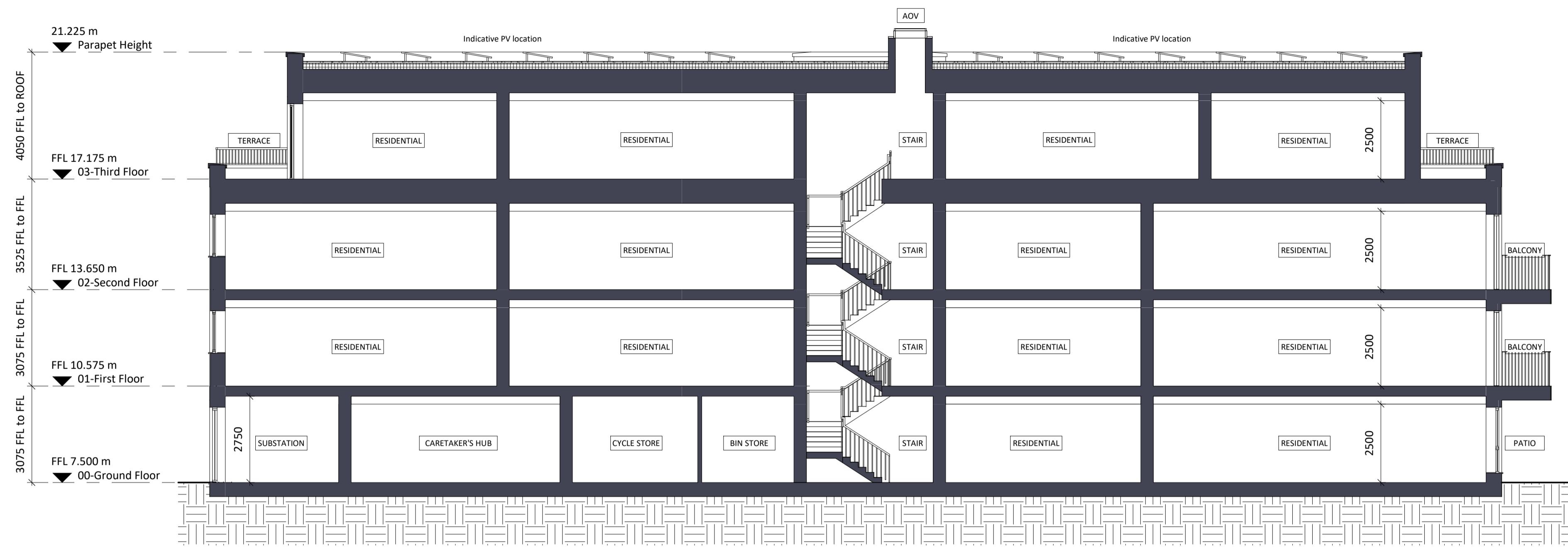
Section AA
