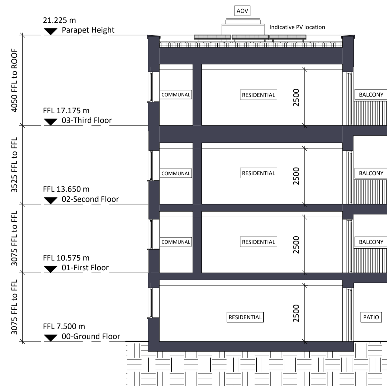
Section BB
