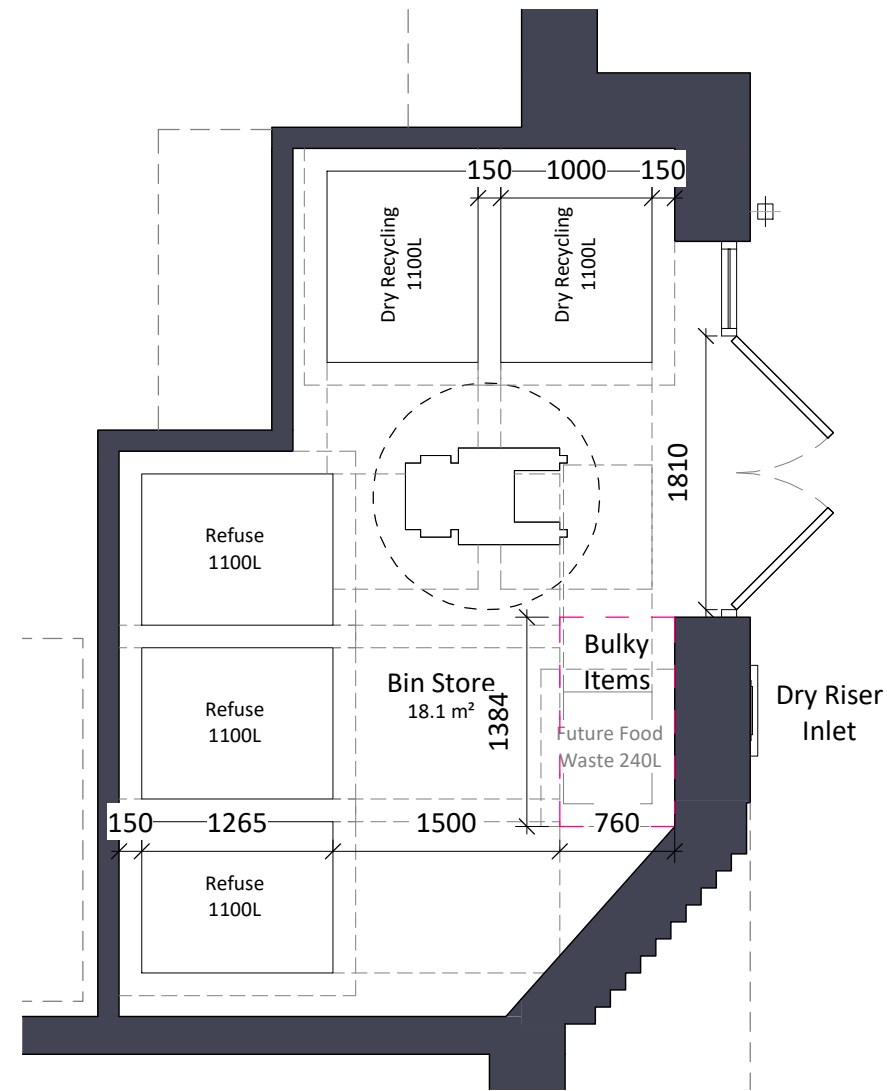
Block B - Refuse Store
