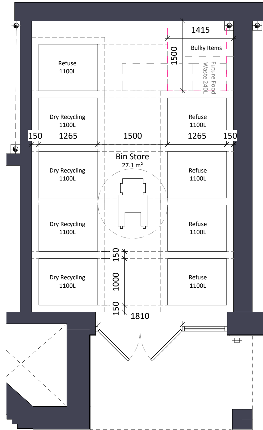
Block C - Refuse Store
