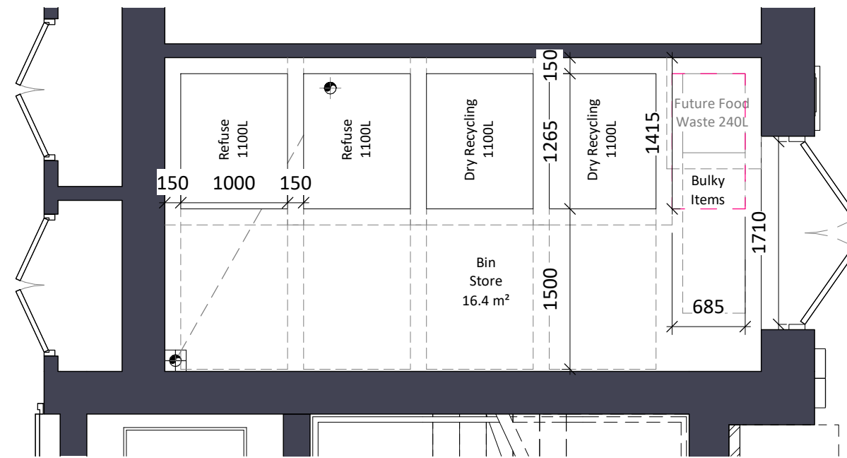
Block W - Refuse Store
