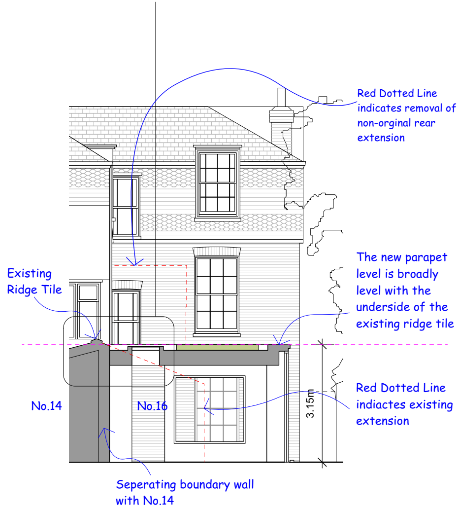
1 Proposed Rear Section B Scale: 1:100
