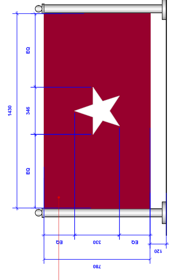
Sign Type H Front Elevation Scale 1:10 @ A1
