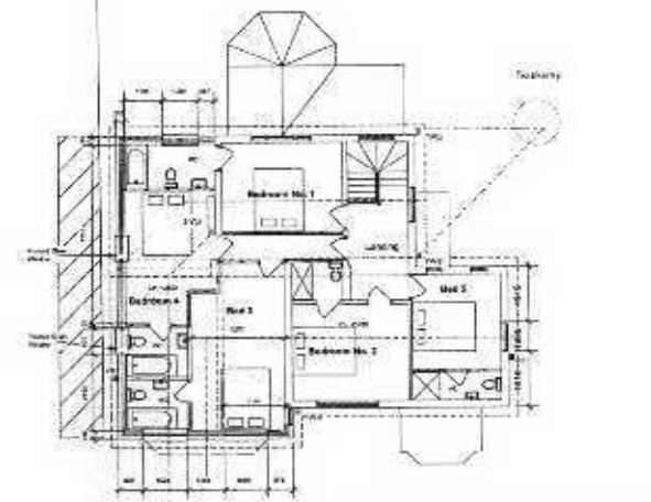
PROPOSED FIRST FLOOR PLAN 1:100
