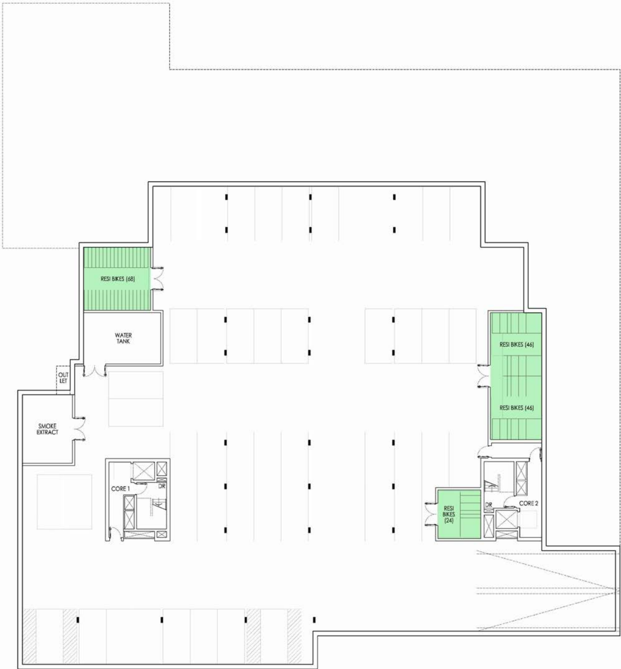
BLOCK B1: BASEMENT PLAN
