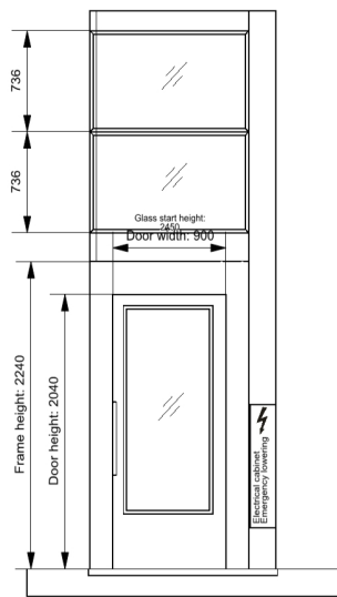
View A
