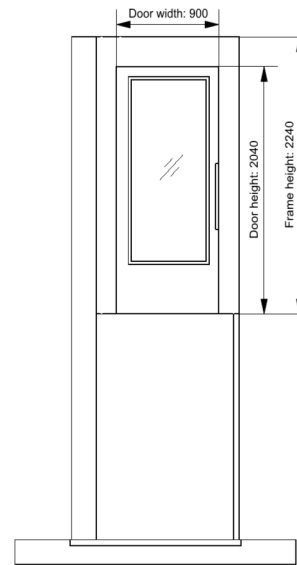
View C
