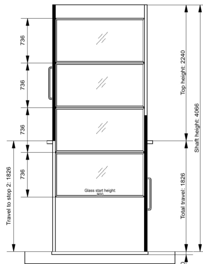
View B
