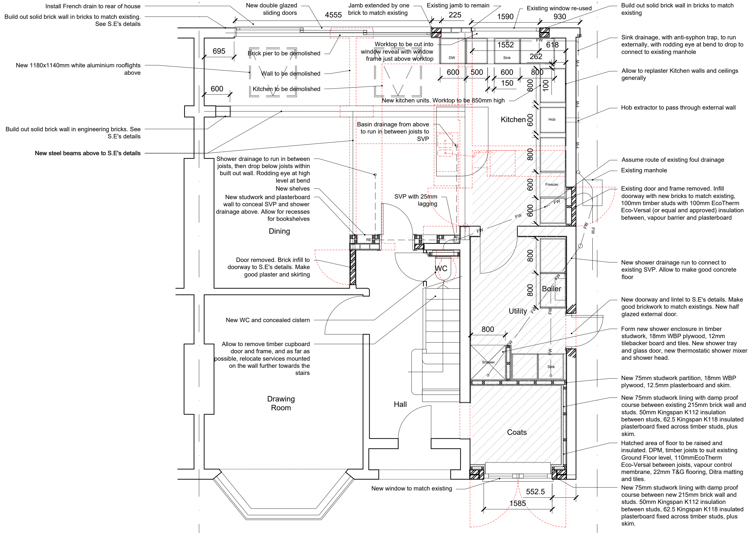
1 PROPOSED GROUND FLOOR PLAN 2001 1:50 @ A3
