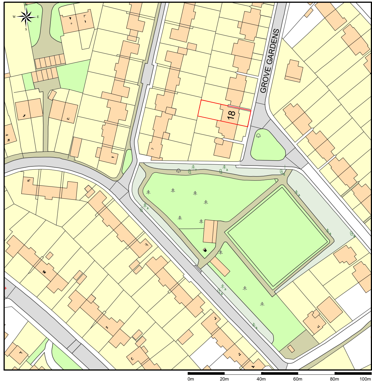
1 EXISTING LOCATION PLAN 0000 1:1250 @ A3
