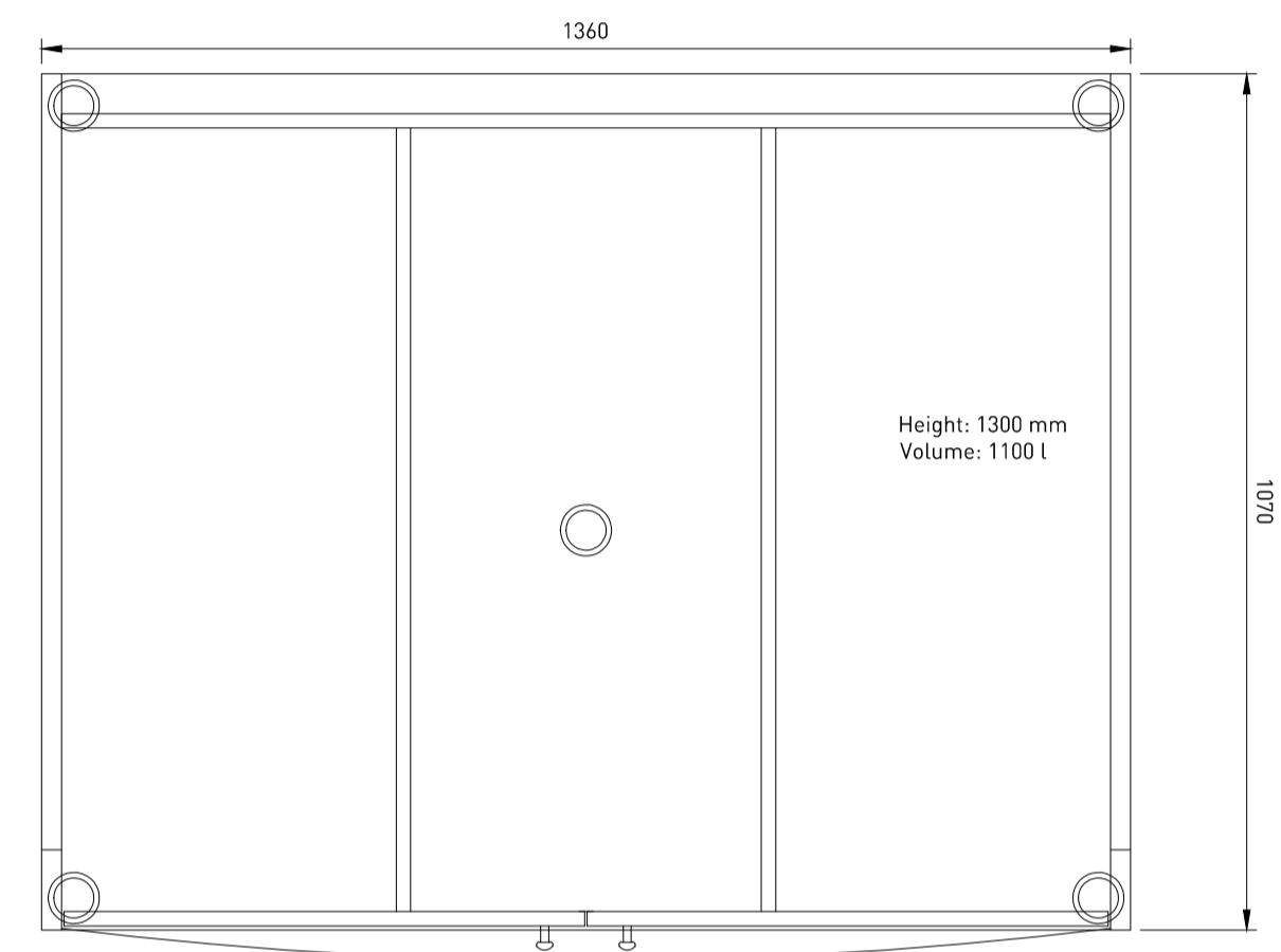
02 1100L BIN DIMENSIONS 1:10
