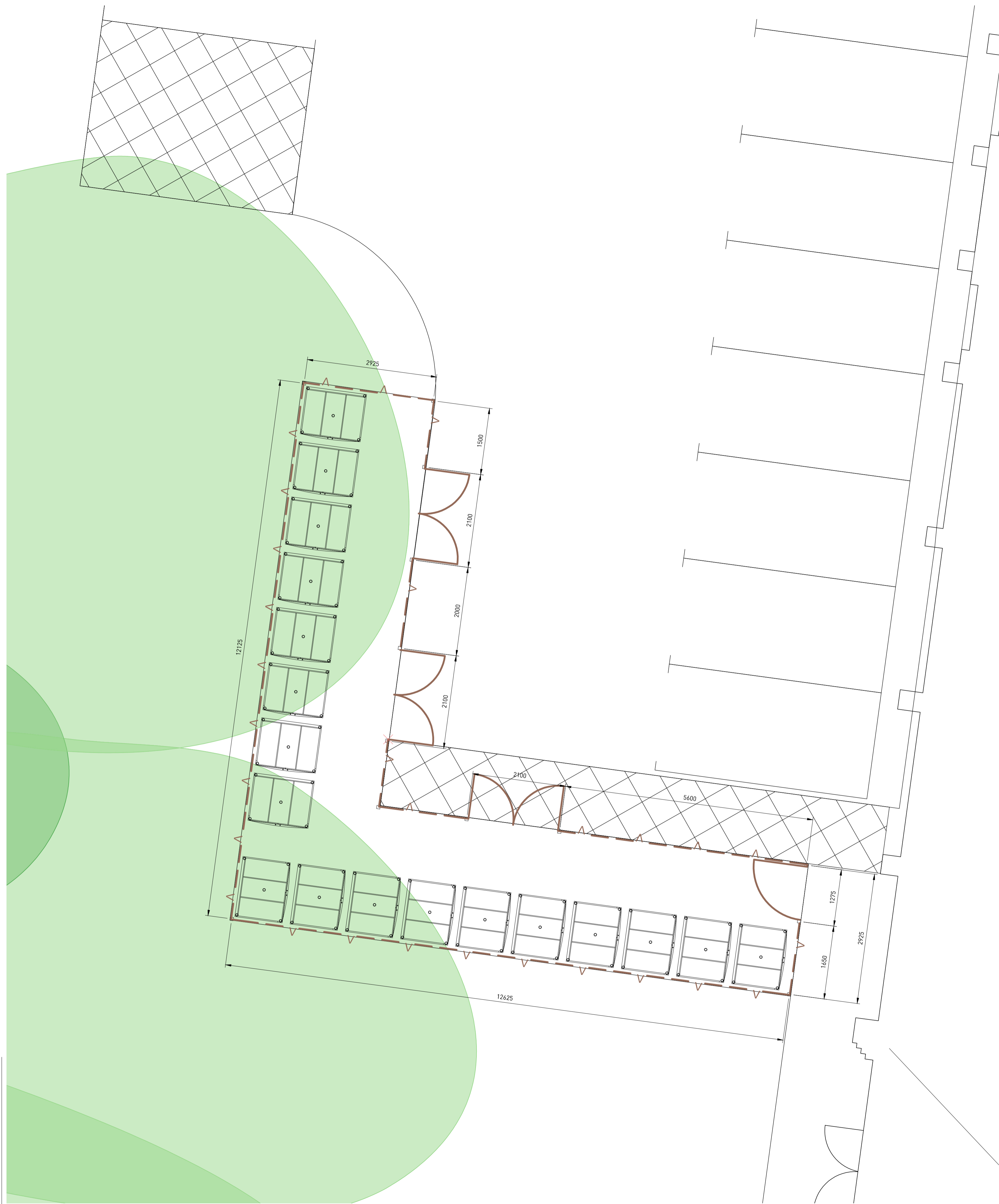
01 BIN STORE GENERAL ARRANGEMENT 1:100
