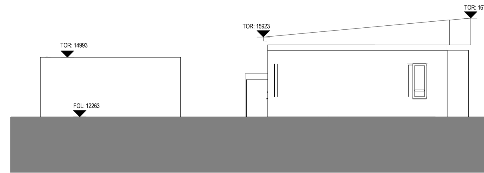
4 EXISTING WEST ELEVATION 1 : 100
