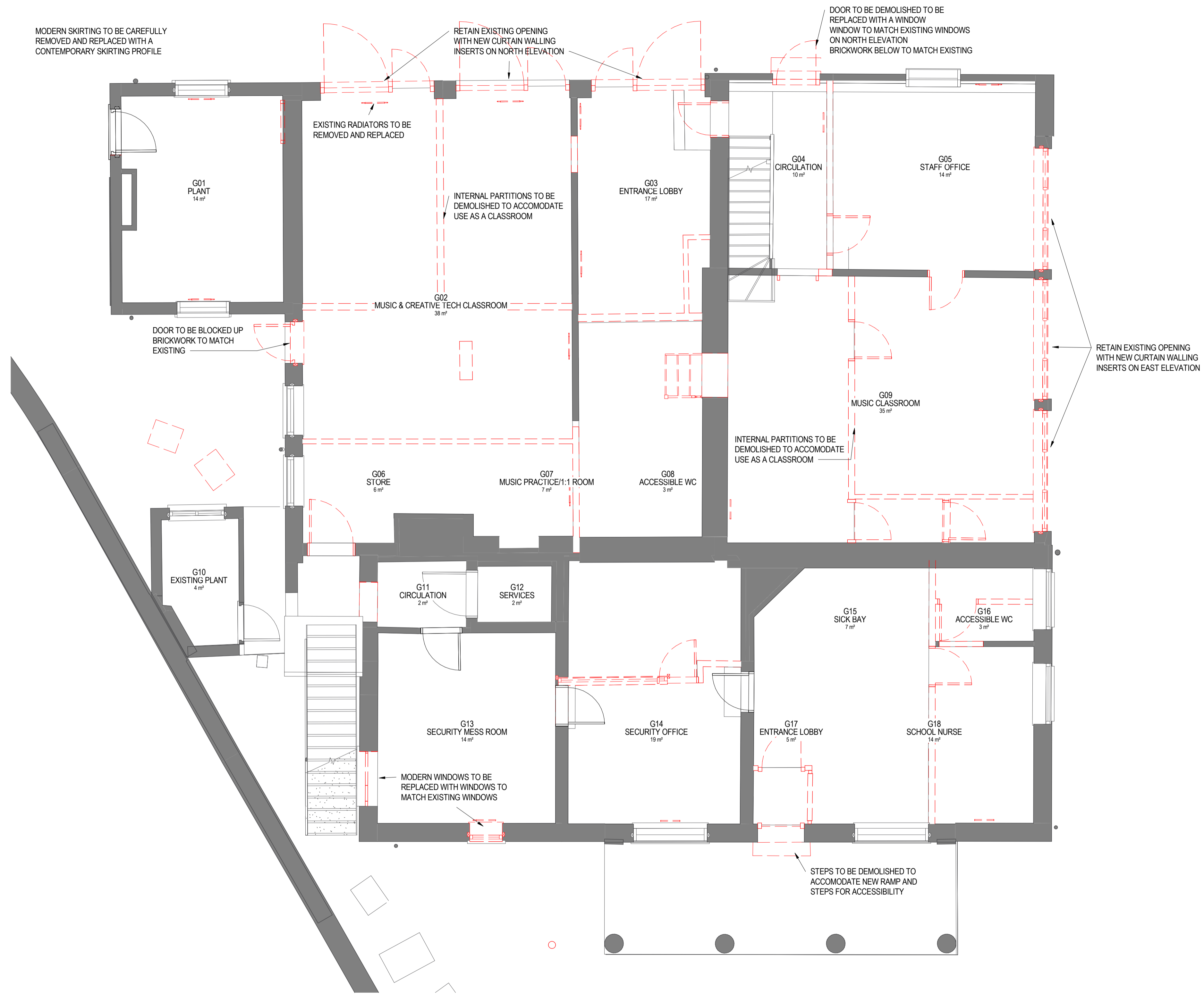
1 GROUND FLOOR DEMOLISHED 1 : 50
