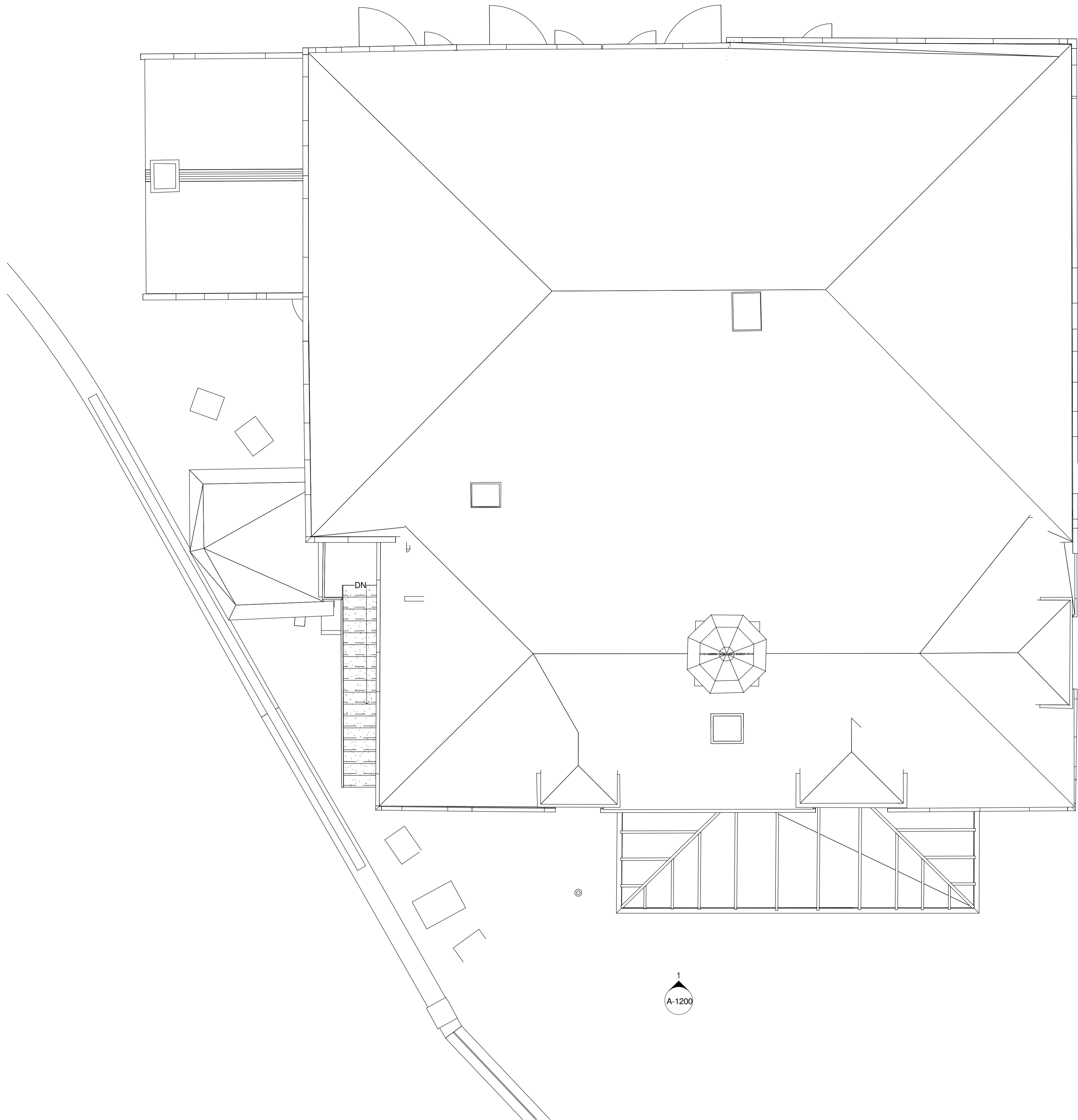
1 ROOF PLAN EXISTING 1 : 50
