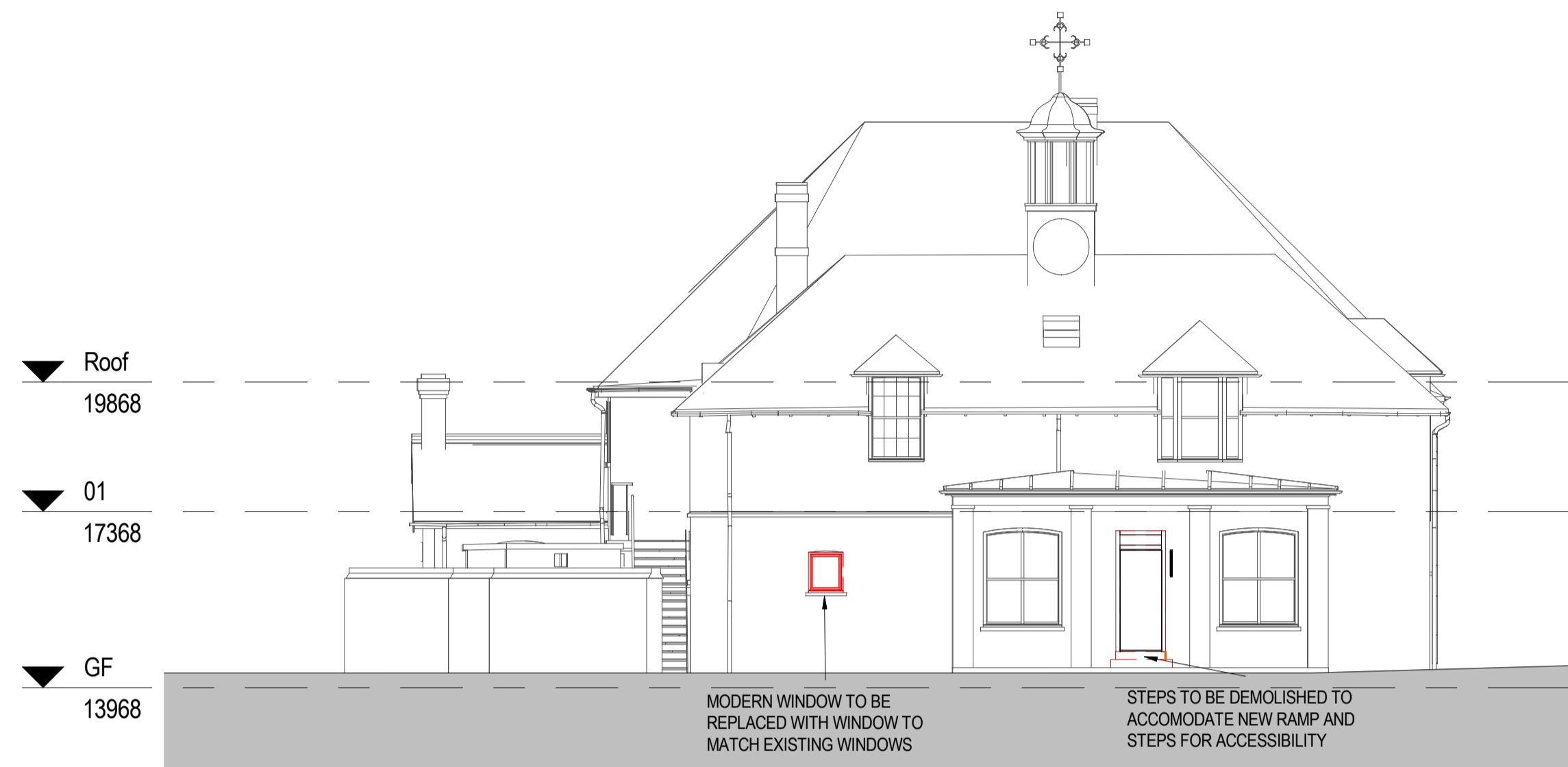
1 SOUTH ELEVATION - DEMOLISHED 1 : 100
