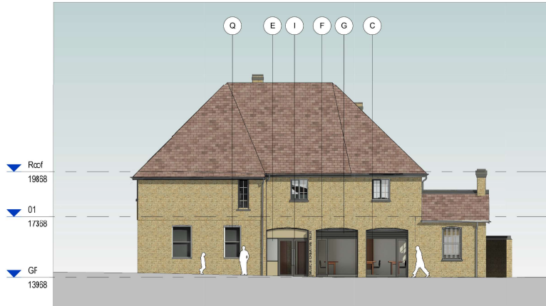
3 NORTH ELEVATION - PROPOSED 1 : 100
