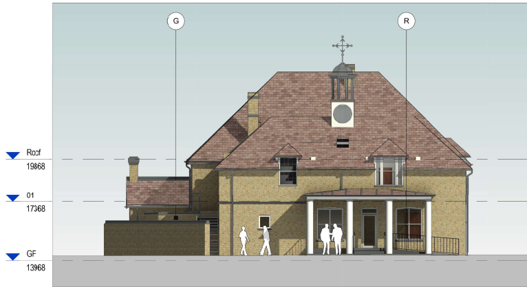
1 SOUTH ELEVATION - PROPOSED 1 : 100
