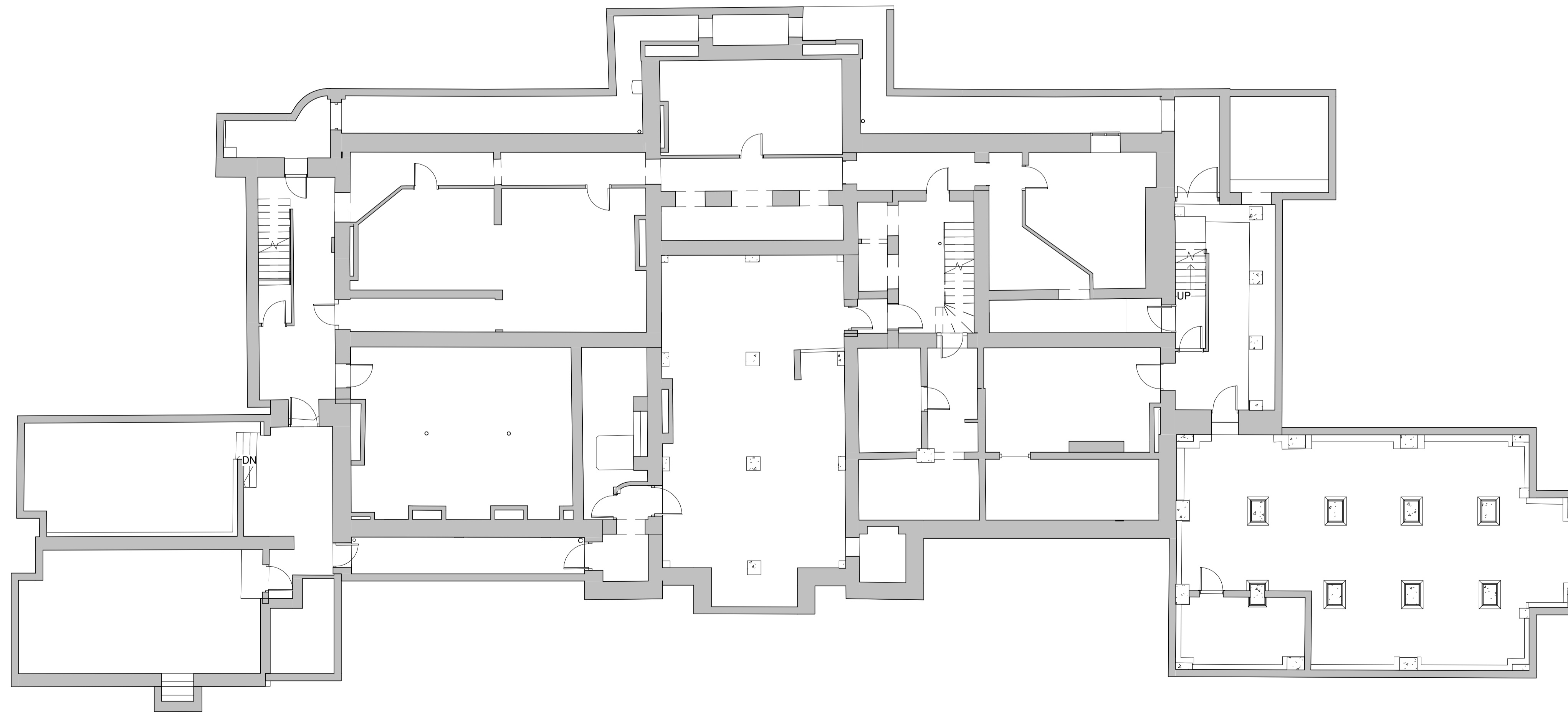
1 LEVEL B1 EXISTING 1 : 100
