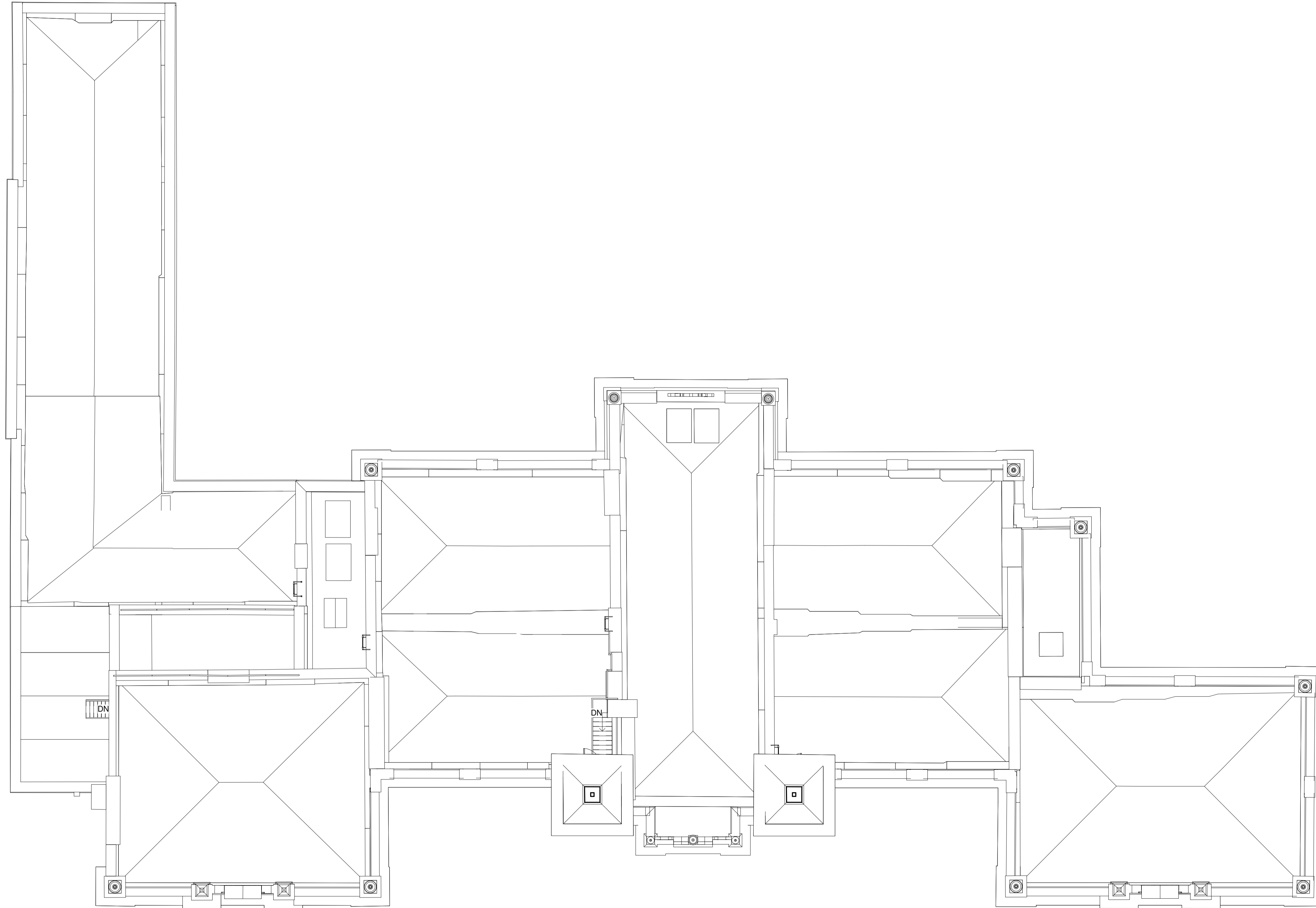
1 ROOF PLAN EXISTING 1 : 100
