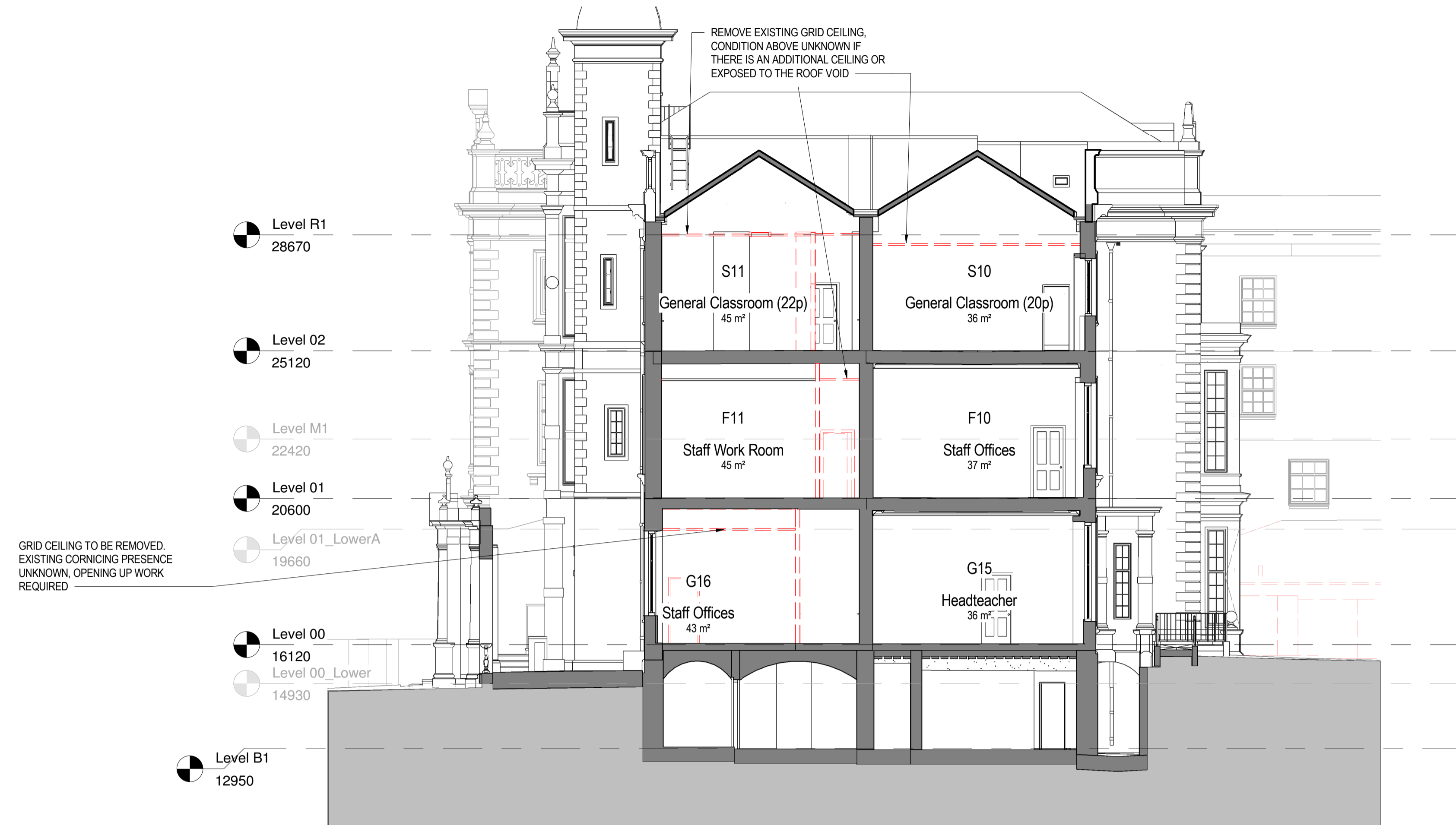
1 SECTION EE - DEMOLISHED 1 : 100
