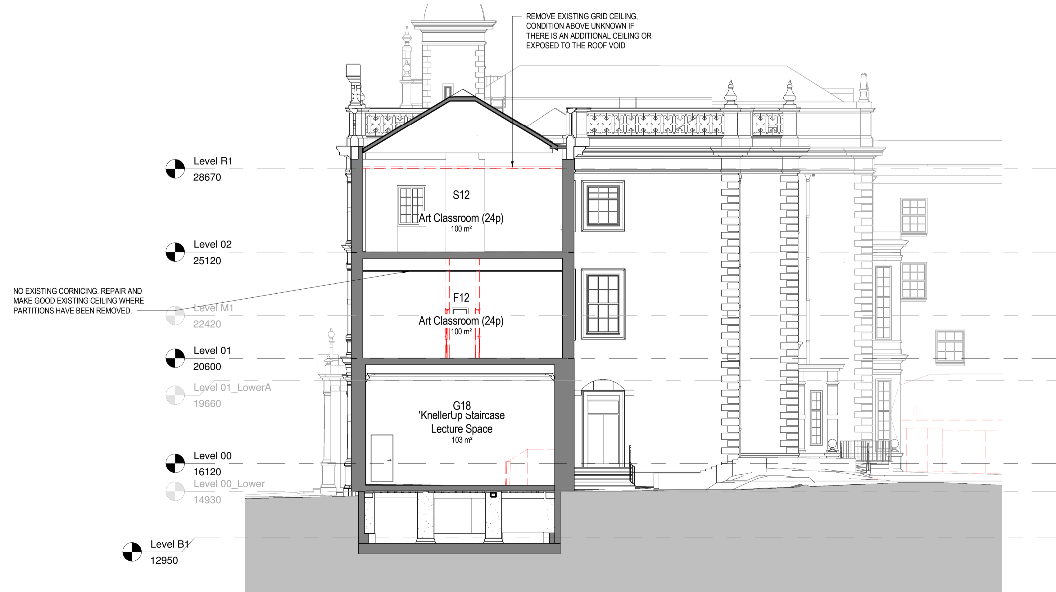
2 SECTION FF - DEMOLISHED 1 : 100
