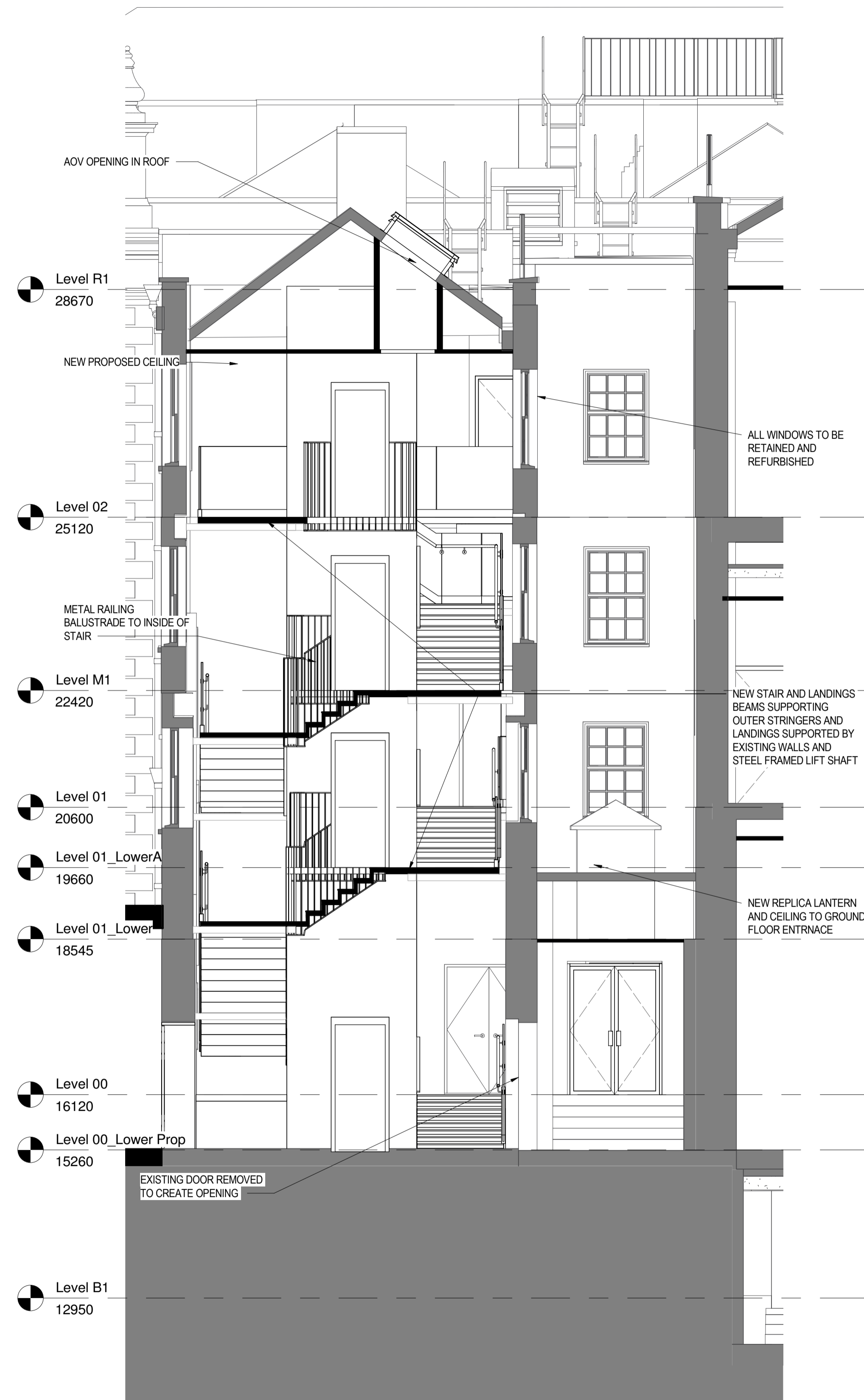
2 SECTION D STAIR - PROPOSED 1 : 50
