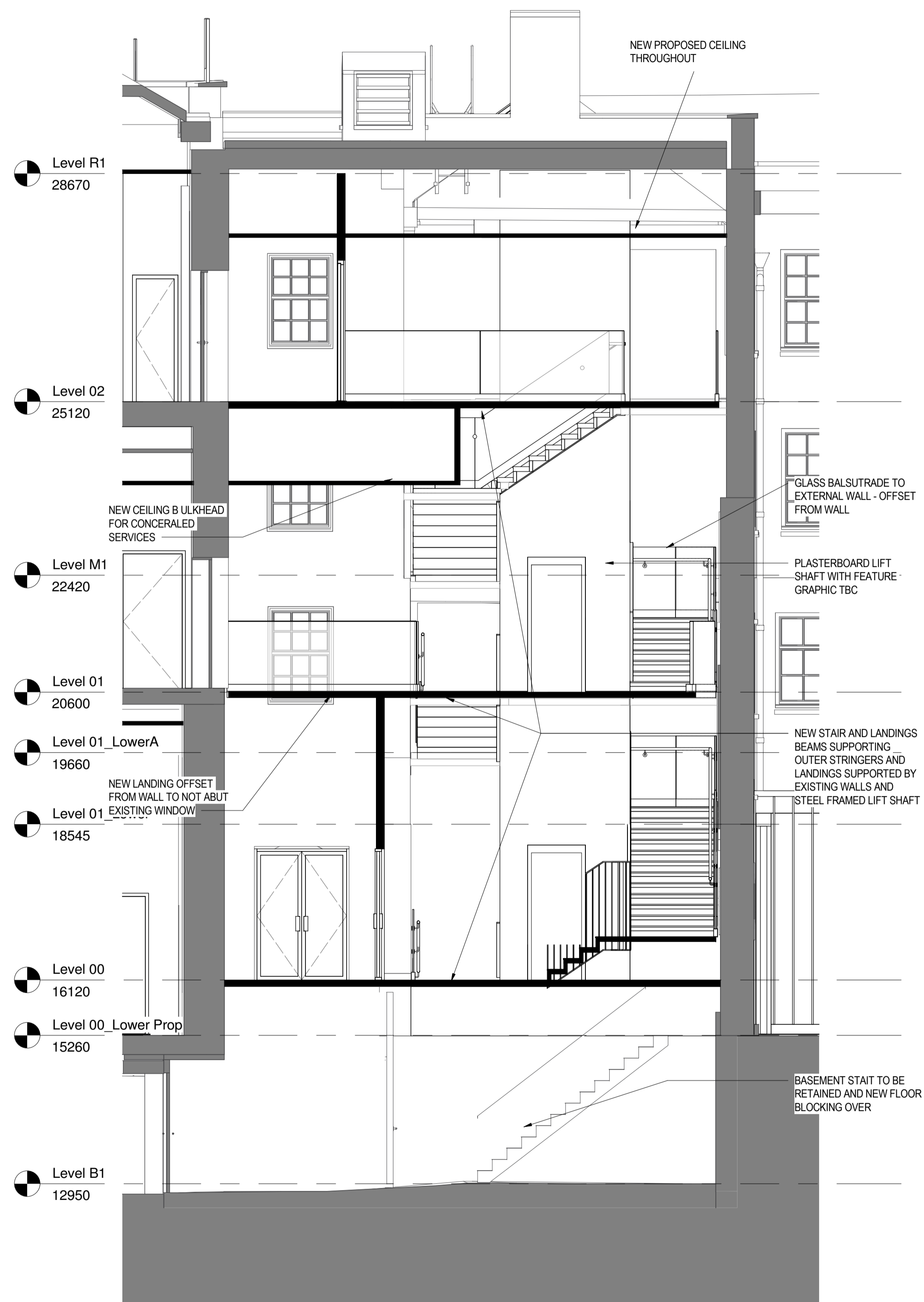
1 SECTION C STAIR - PROPOSED 1 : 50
