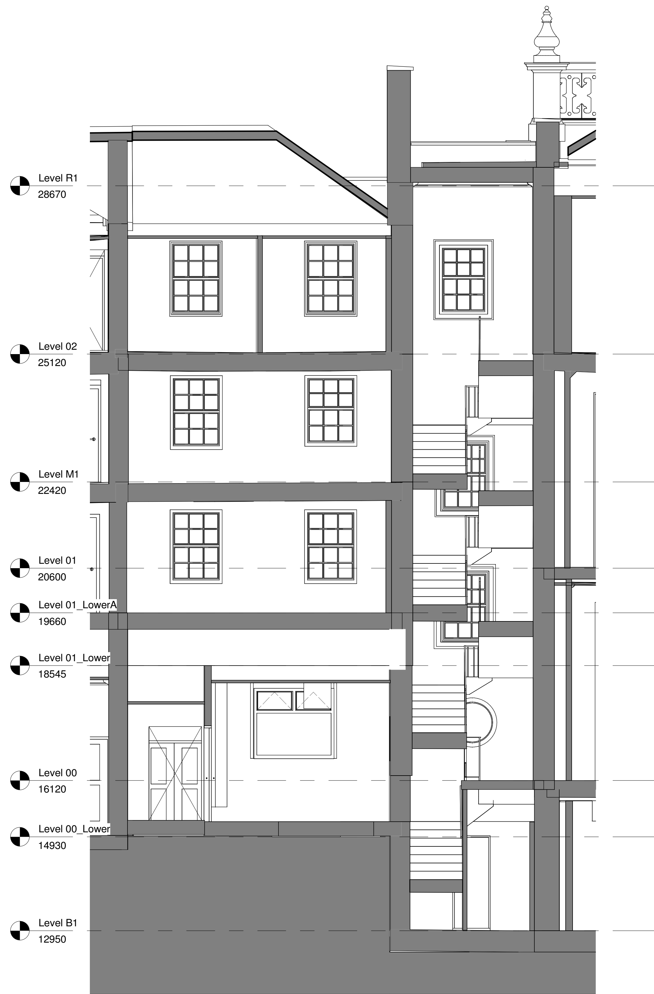
1 SECTION A STAIR EXISTING 1 : 50
