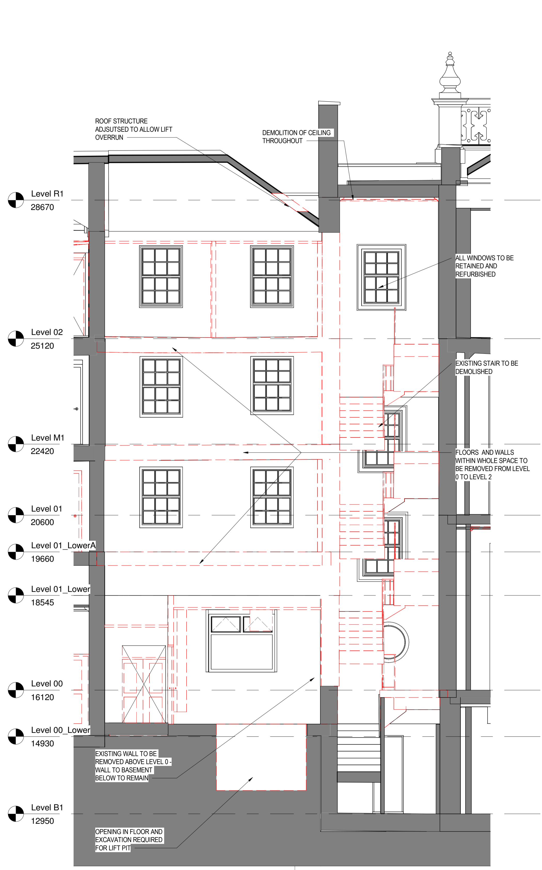
1 SECTION A STAIR DEMOLITION 1 : 50
