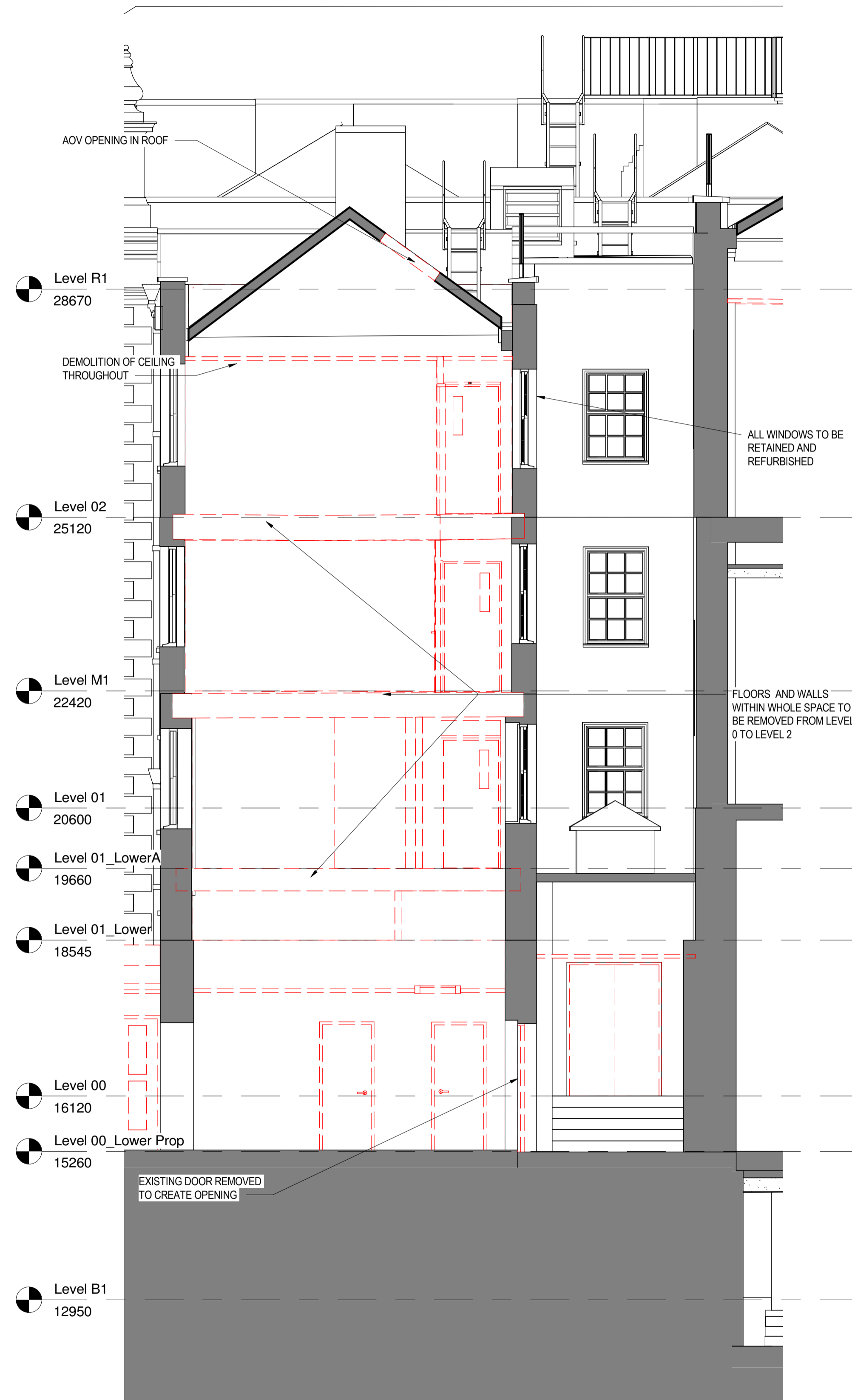
2 SECTION D STAIR - DEMOLITION 1:50
