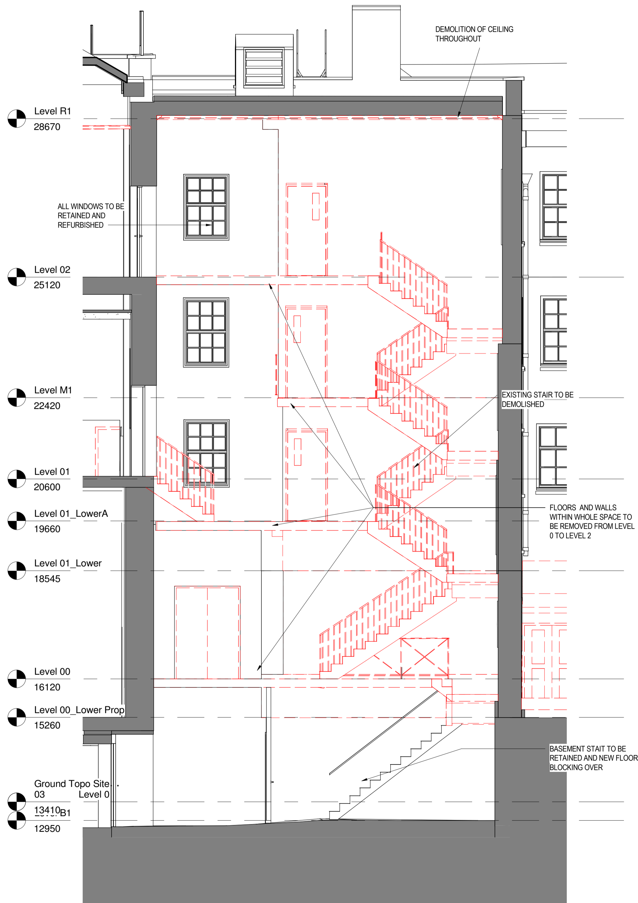
1 SECTION C STAIR - DEMOLITION 1:50
