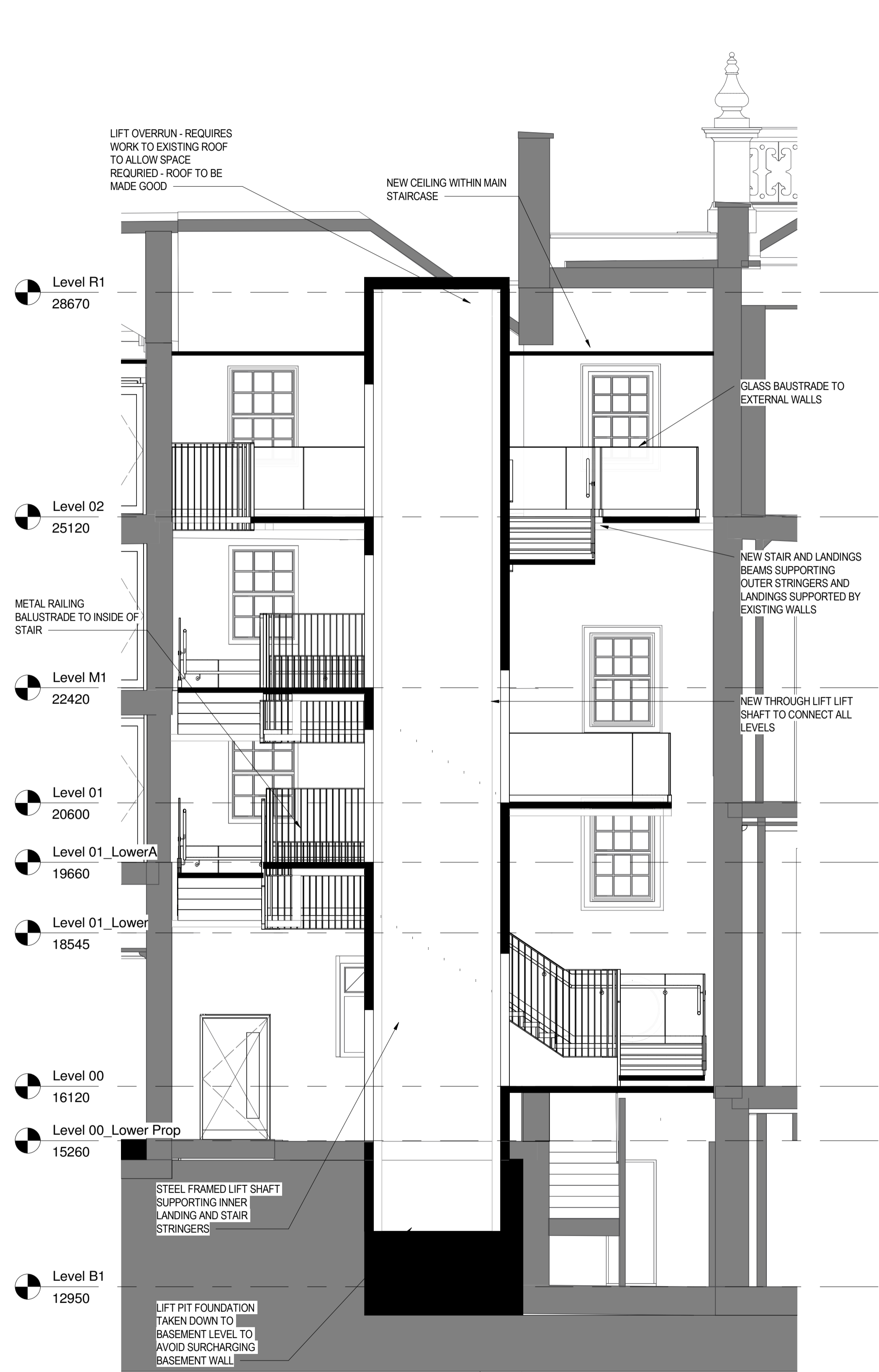
1 SECTION A STAIR PROPOSED 1 : 50
