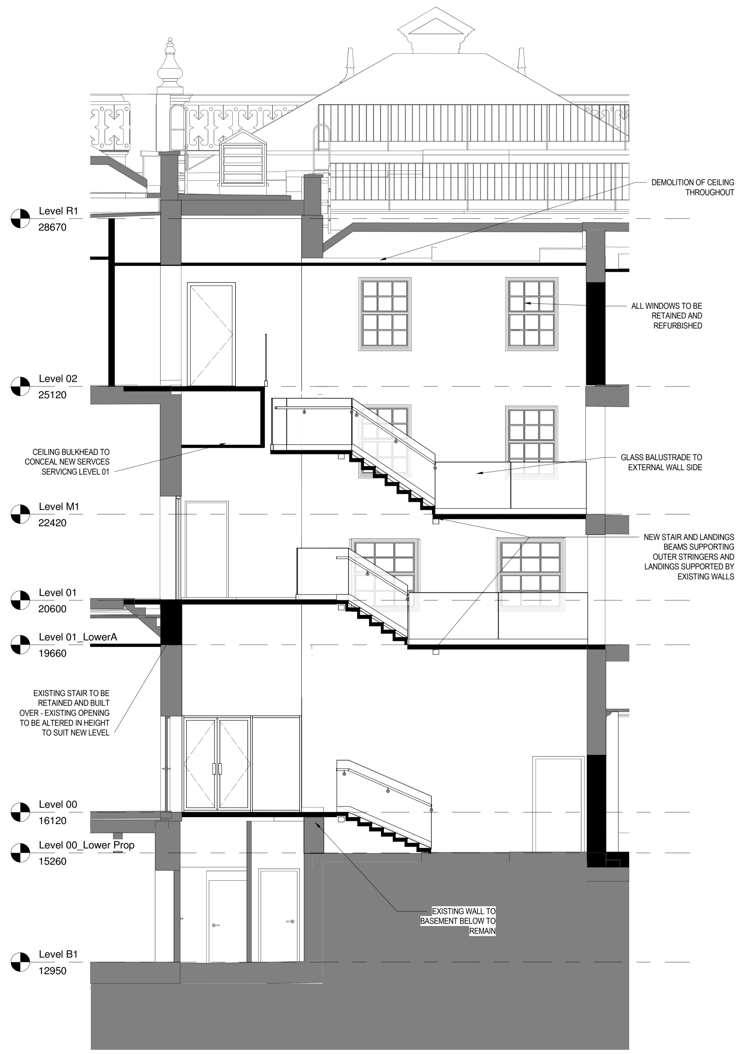
2 SECTION B STAIR - PROPOSED 1 : 50
