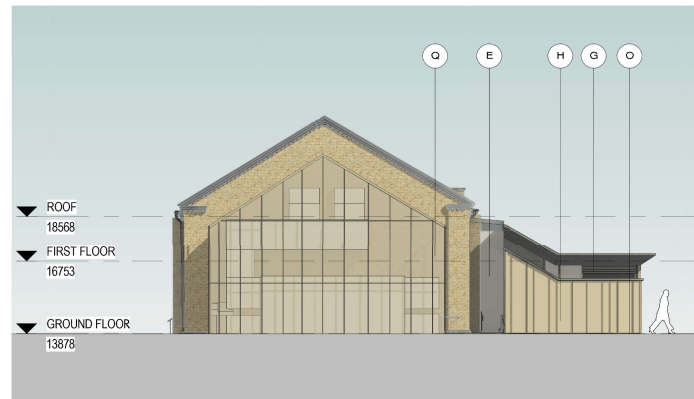
6 WEST ELEVATION - PROPOSED 1 : 100
