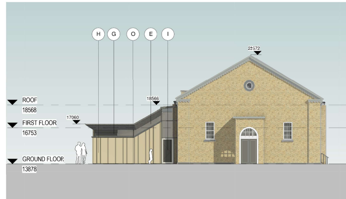
3 EAST ELEVATION - PROPOSED 1 : 100
