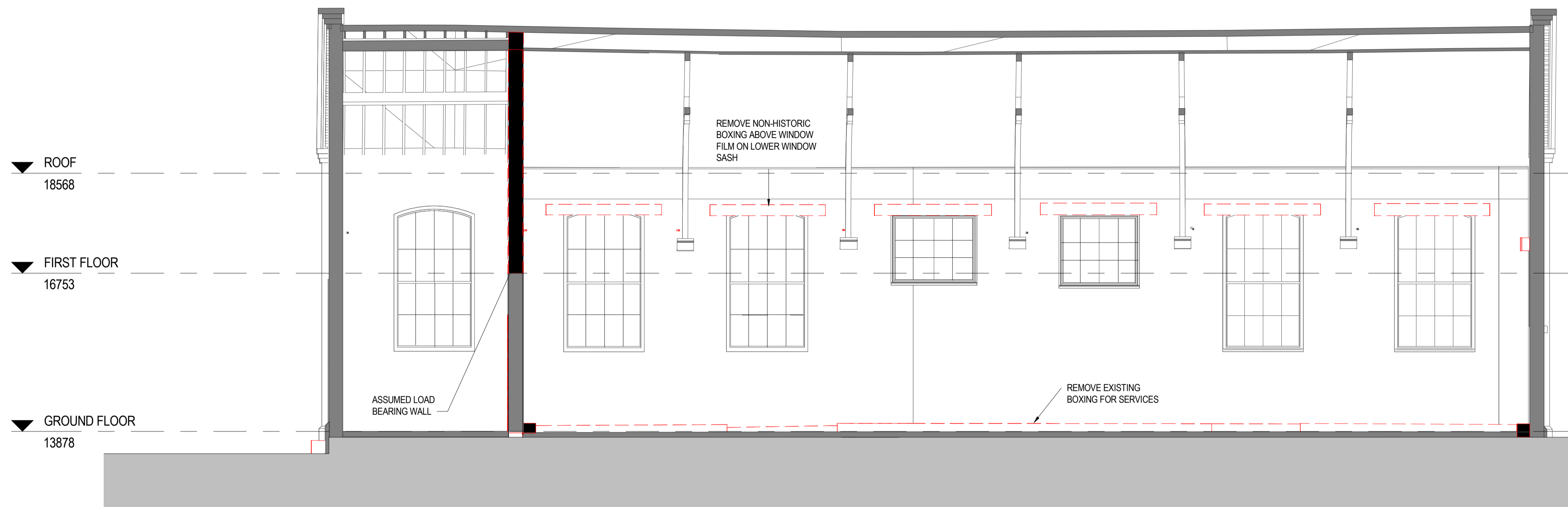
1 LONG SECTION AA - DEMOLISHED 1 : 50
