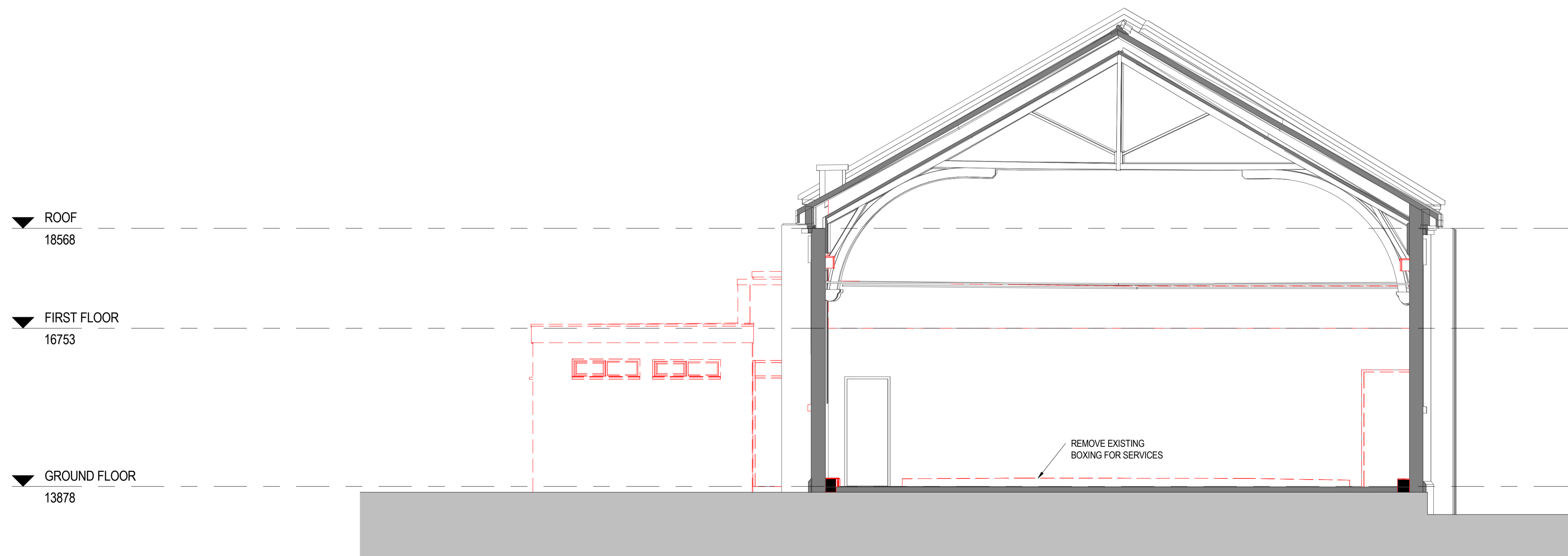
2 SHORT SECTION BB - DEMOLISHED 1 : 50
