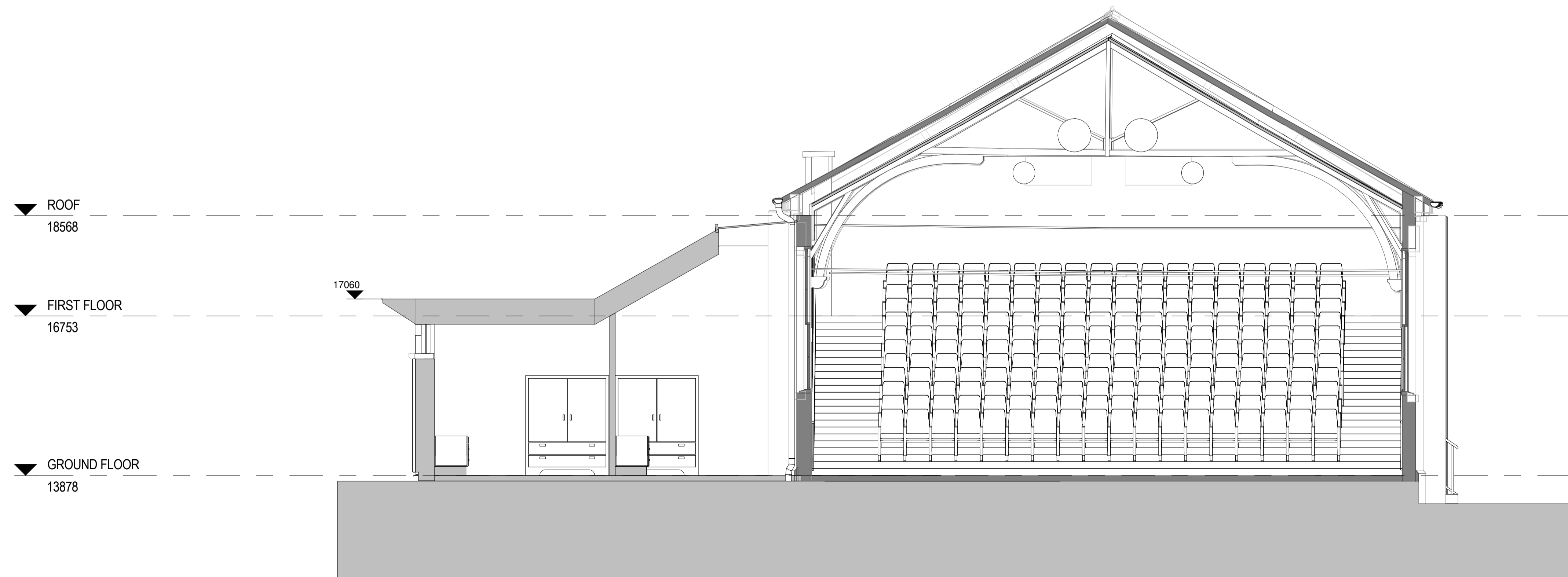
2 SHORT SECTION BB 1 : 50
