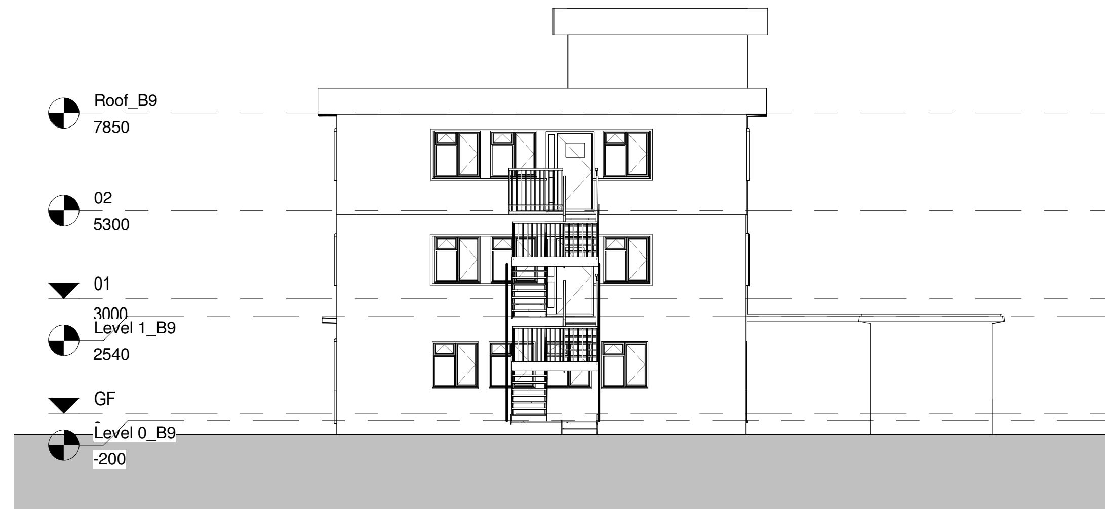
1 NORTH ELEVATION 1 : 100
