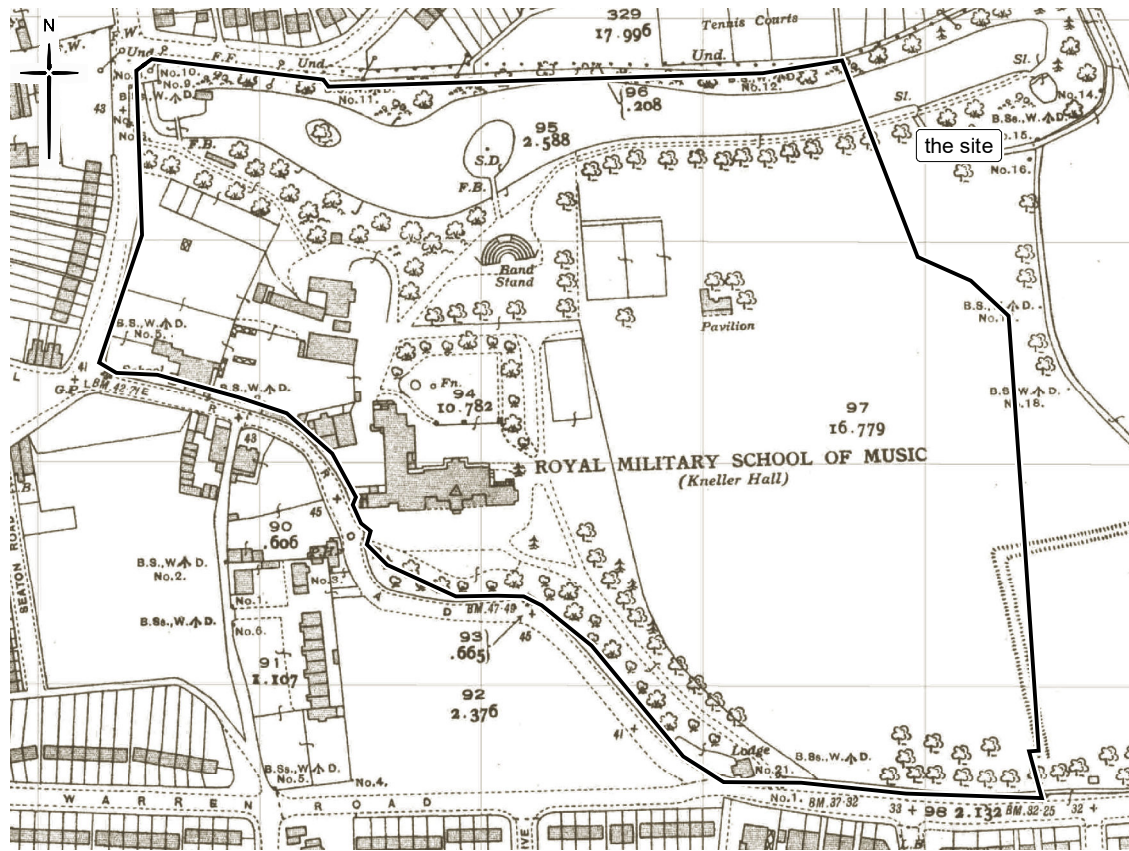
Fig 11 Ordnance Survey 25" : mile map of 1934 (not to scale)
