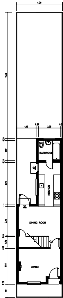
GROUND FLOOR
