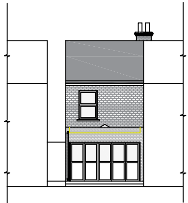
② PROPOSED REAR ELEVATION 1 : 100
