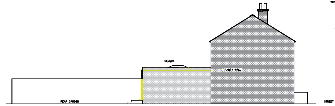
④ PROPOSED SIDE ELEVATION 2 1 : 100
